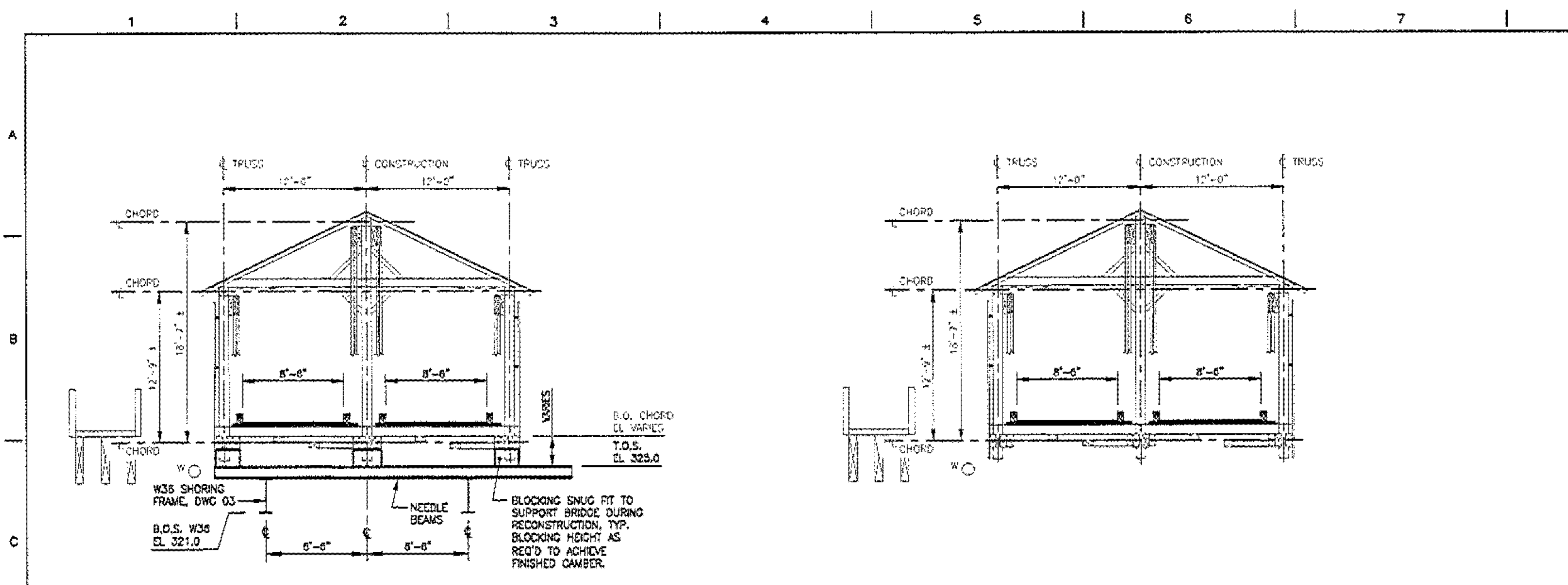
SECTION LOOKING WEST SCALE 0 5 10 FEET
