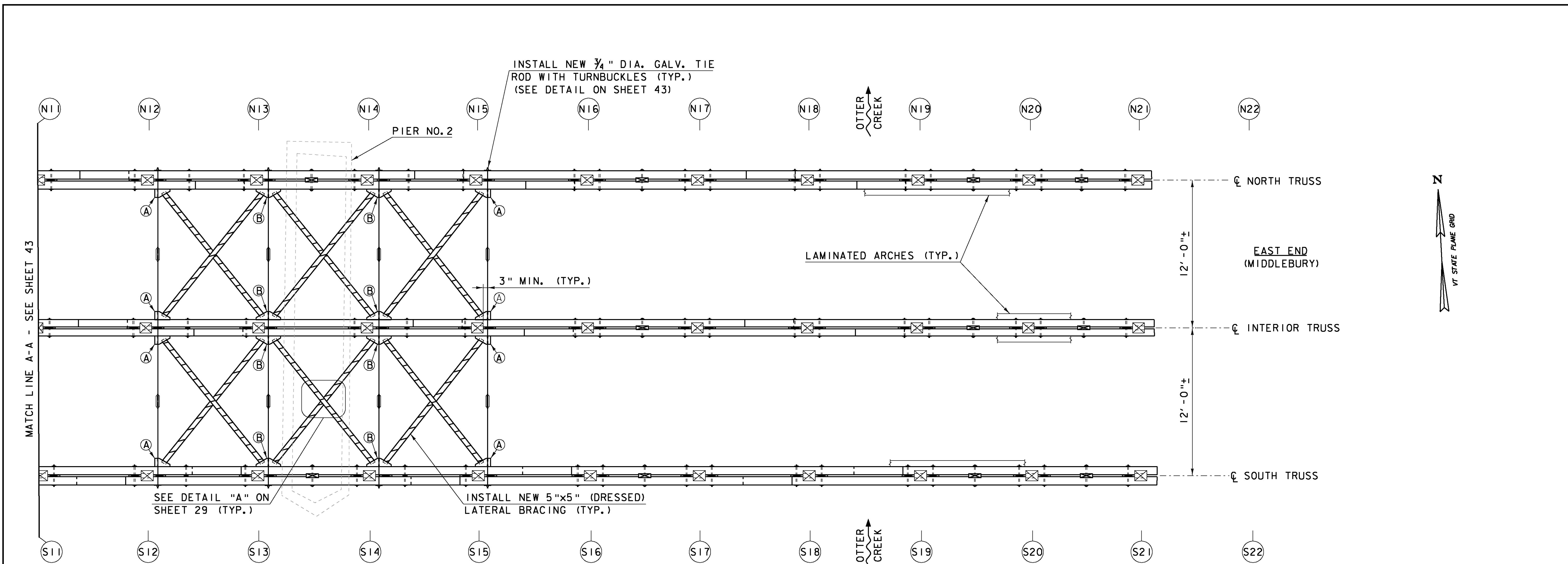
LOWER LATERAL BRACING PLAN SCALE: 1/4" = 1'-0"
