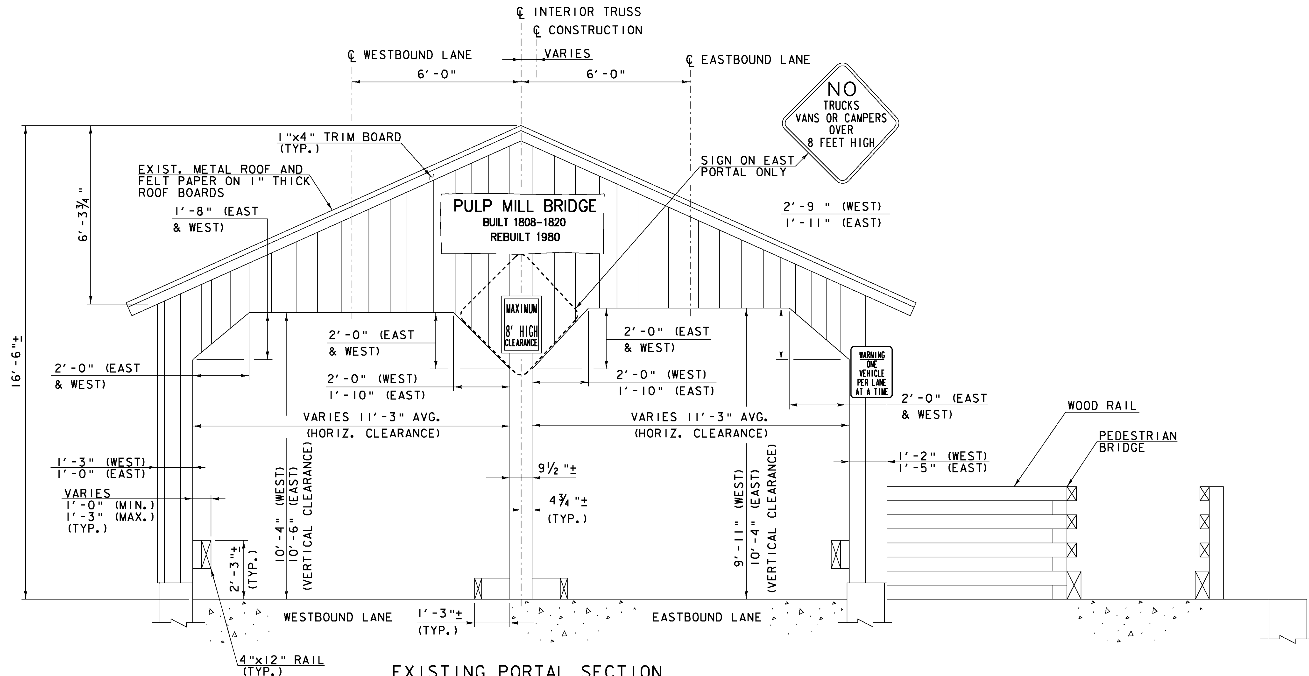
EXISTING PORTAL SECTION (LOOKING EAST) (WEST PORTAL SHOWN, EAST SIMILAR) SCALE: 1/2" = 1'-0"
