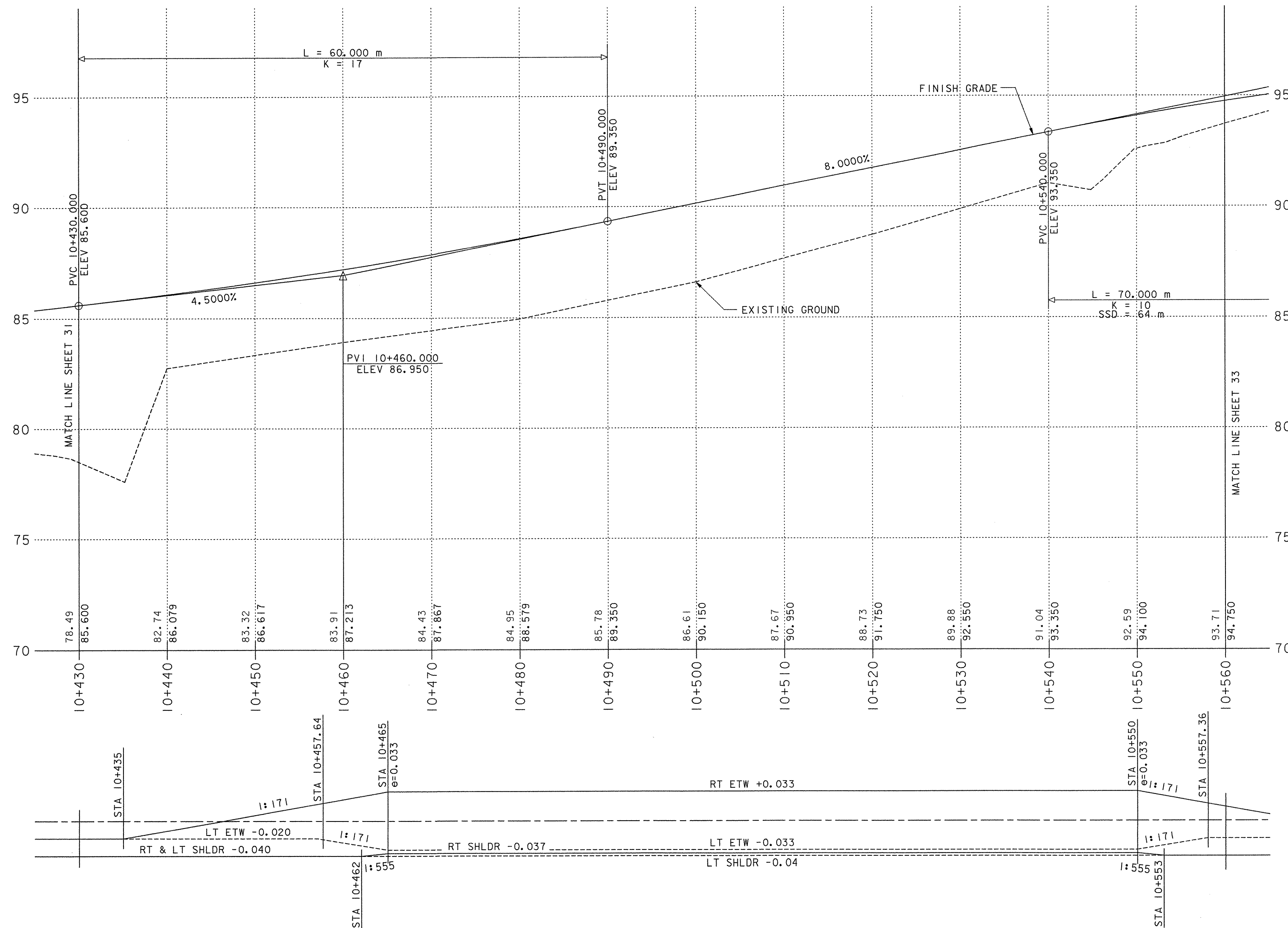
PROFILE & BANKING DIAGRAM
