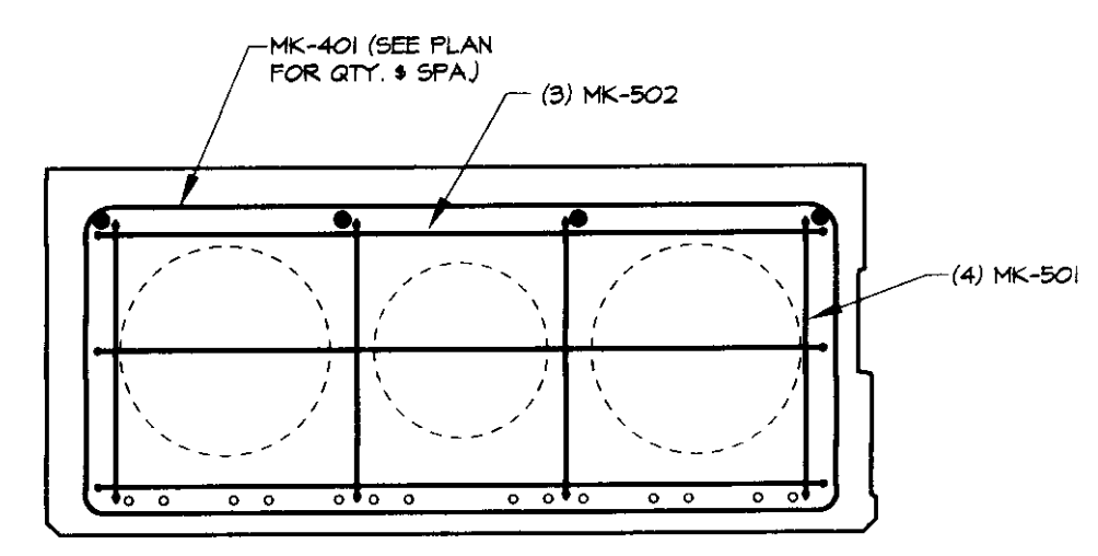
C END BLOCK REINFORCING ELEV. 3/4" = 1'-0"
