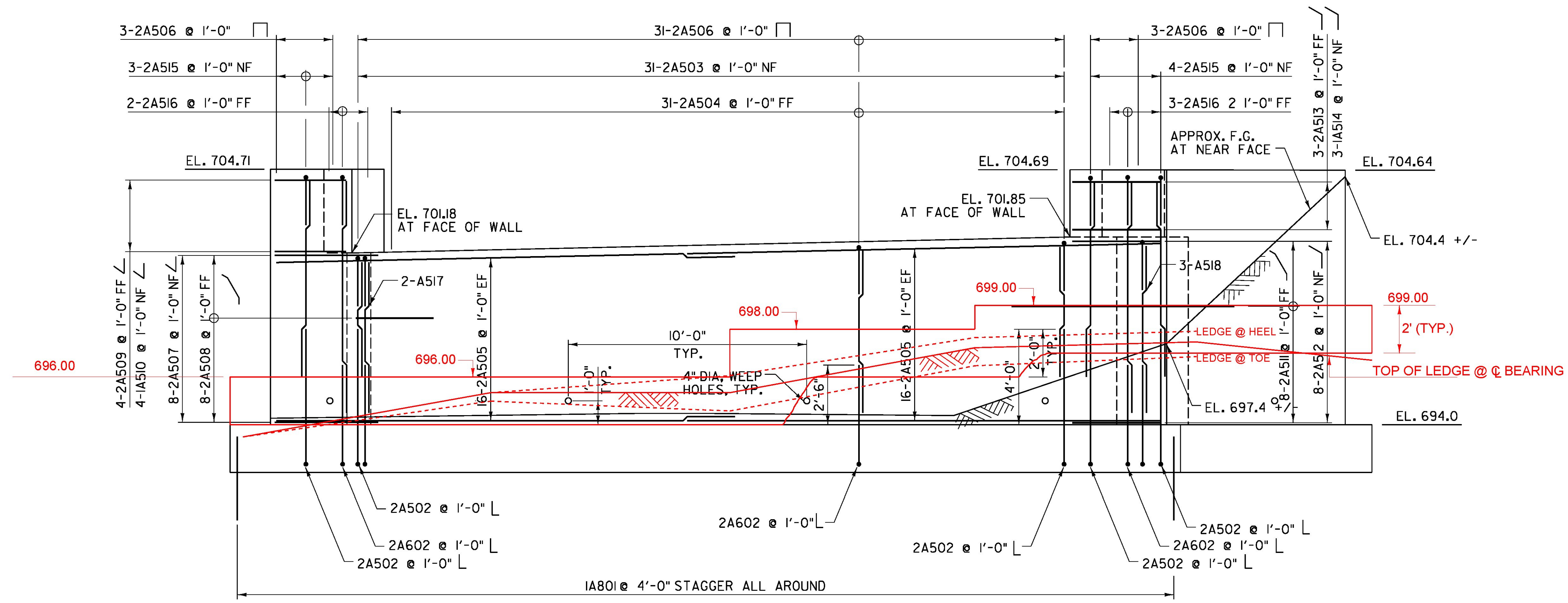
ABUTMENT 2 REINFORCEMENT SCALE 3/8" = 1'-0"
