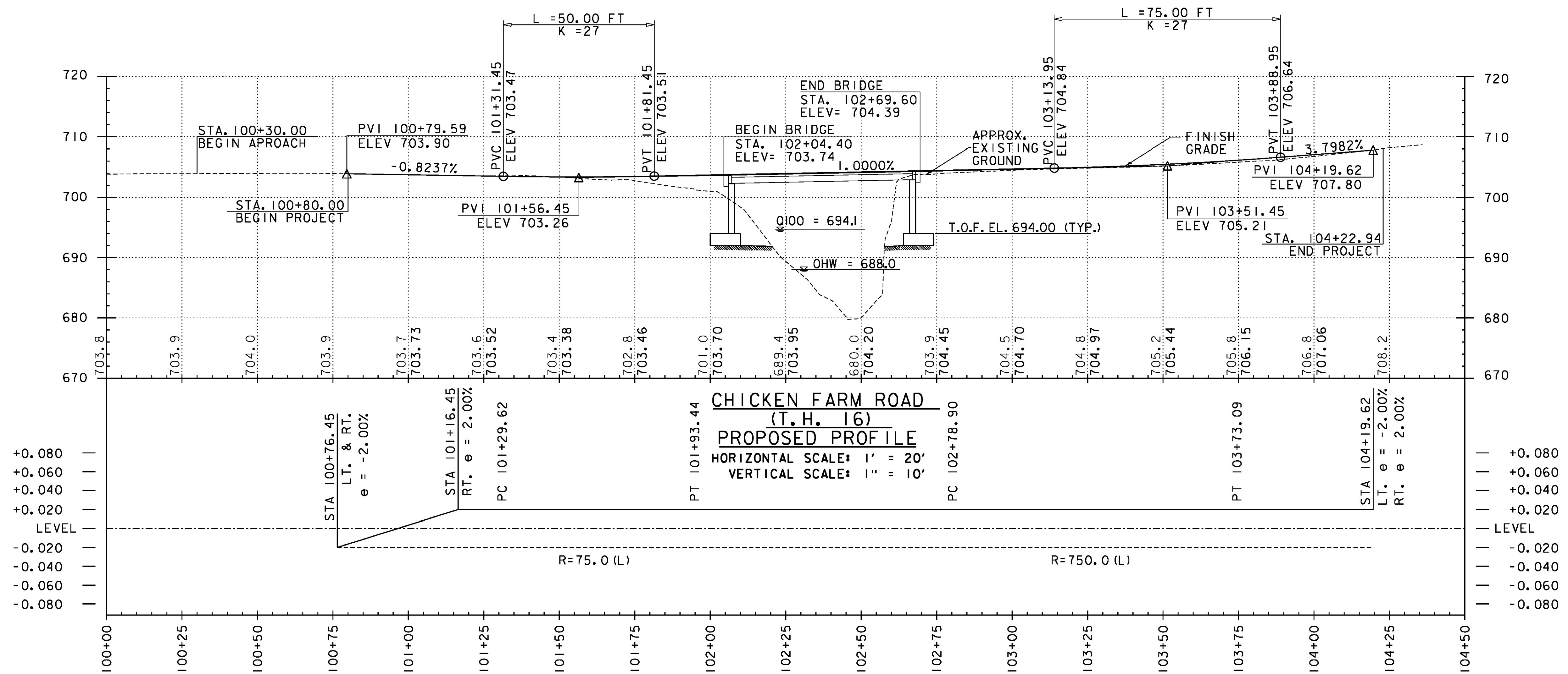
BANKING DIAGRAM HORIZONTAL SCALE: 1" = 20'
