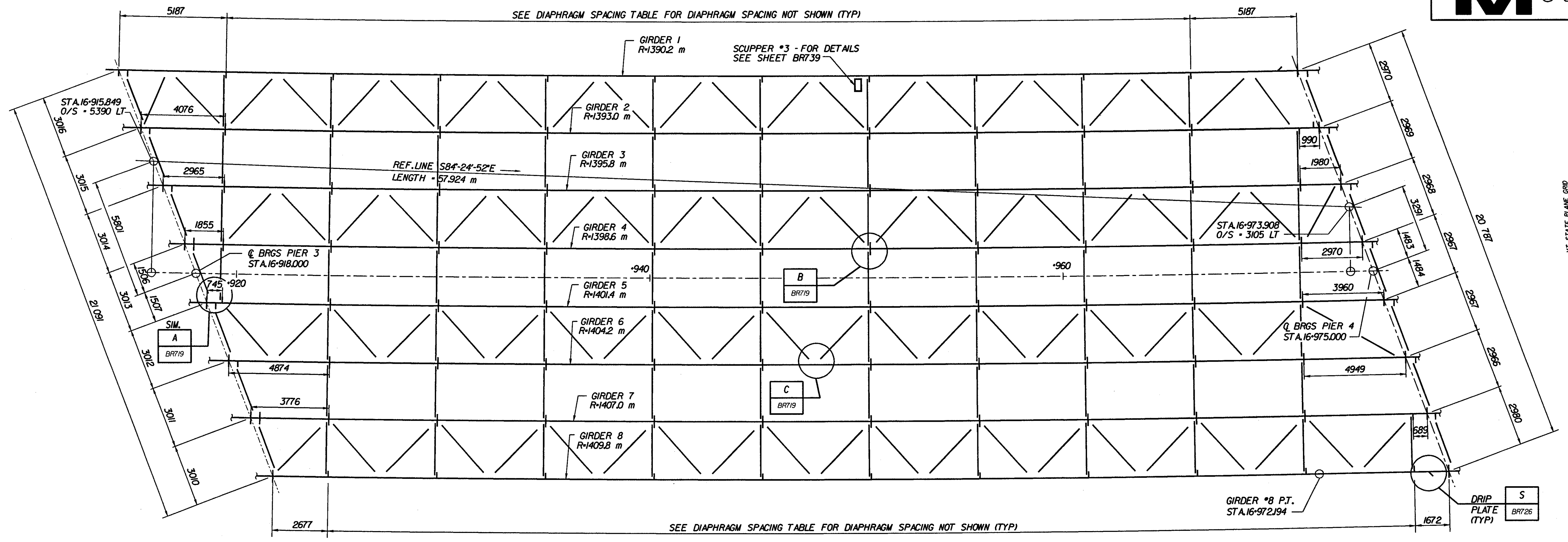
FRAMING PLAN - SPAN 4
