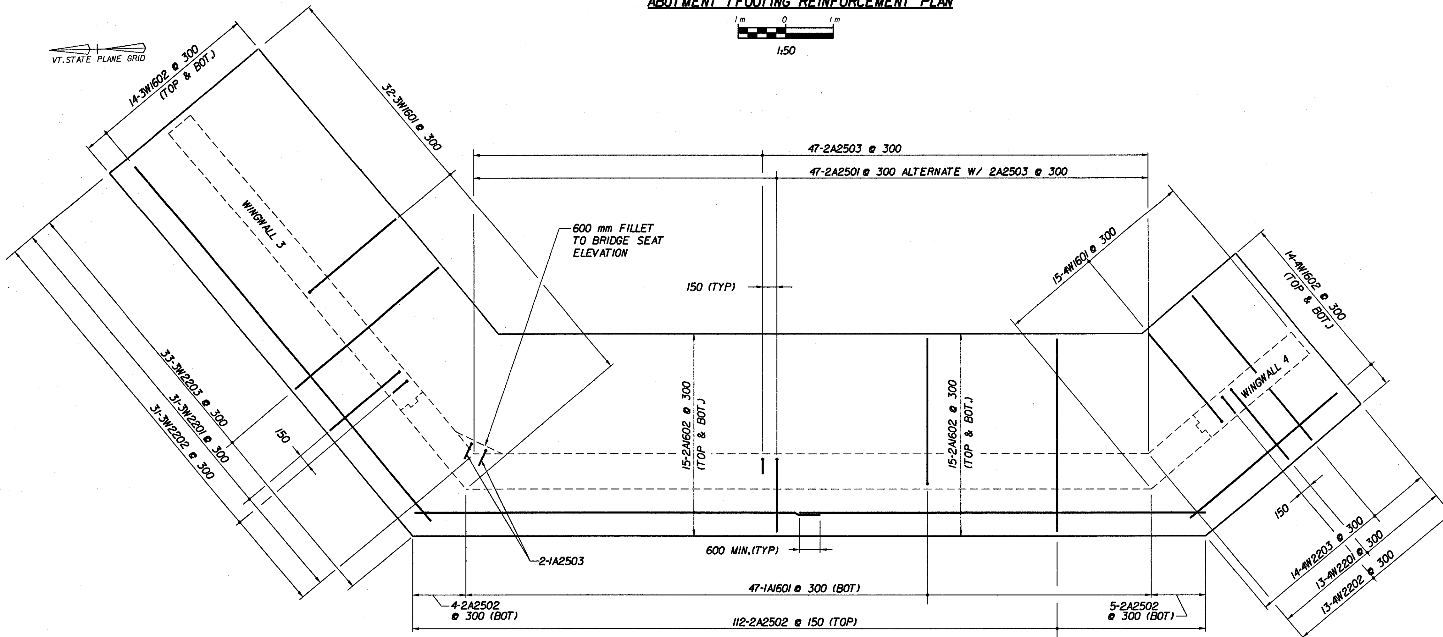
ABUTMENT 2 FOOTING REINFORCEMENT PLAN
