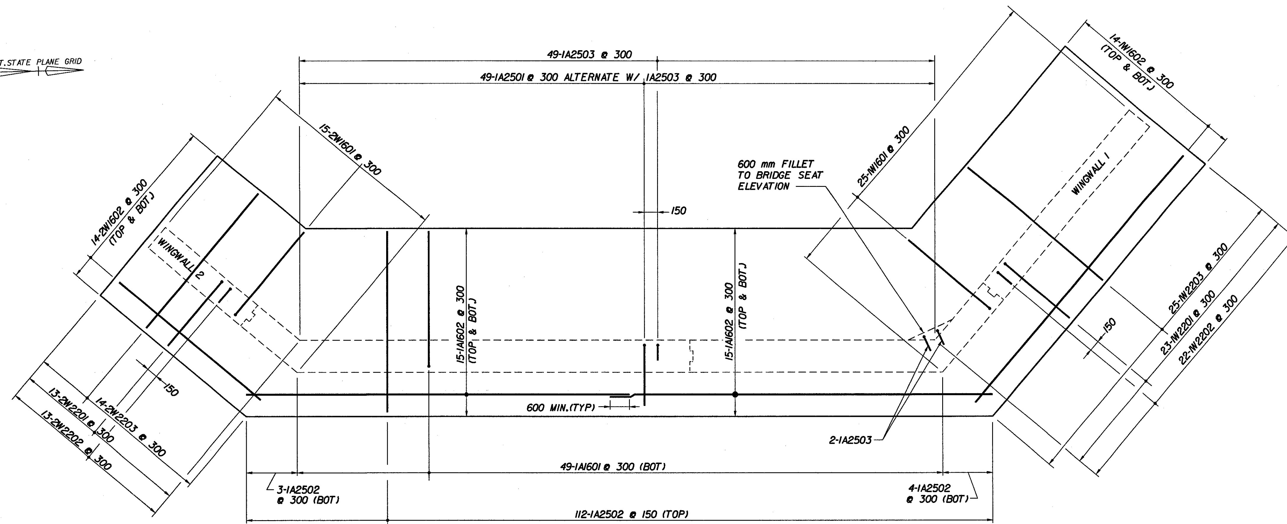
ABUTMENT 1 FOOTING REINFORCEMENT PLAN
