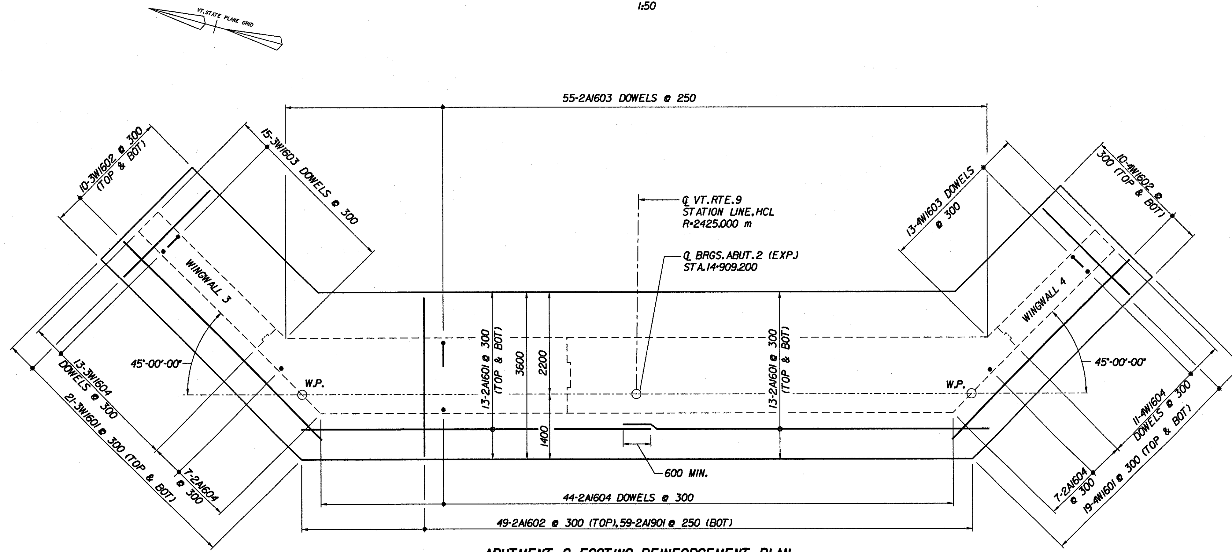
ABUTMENT 2 FOOTING REINFORCEMENT PLAN
