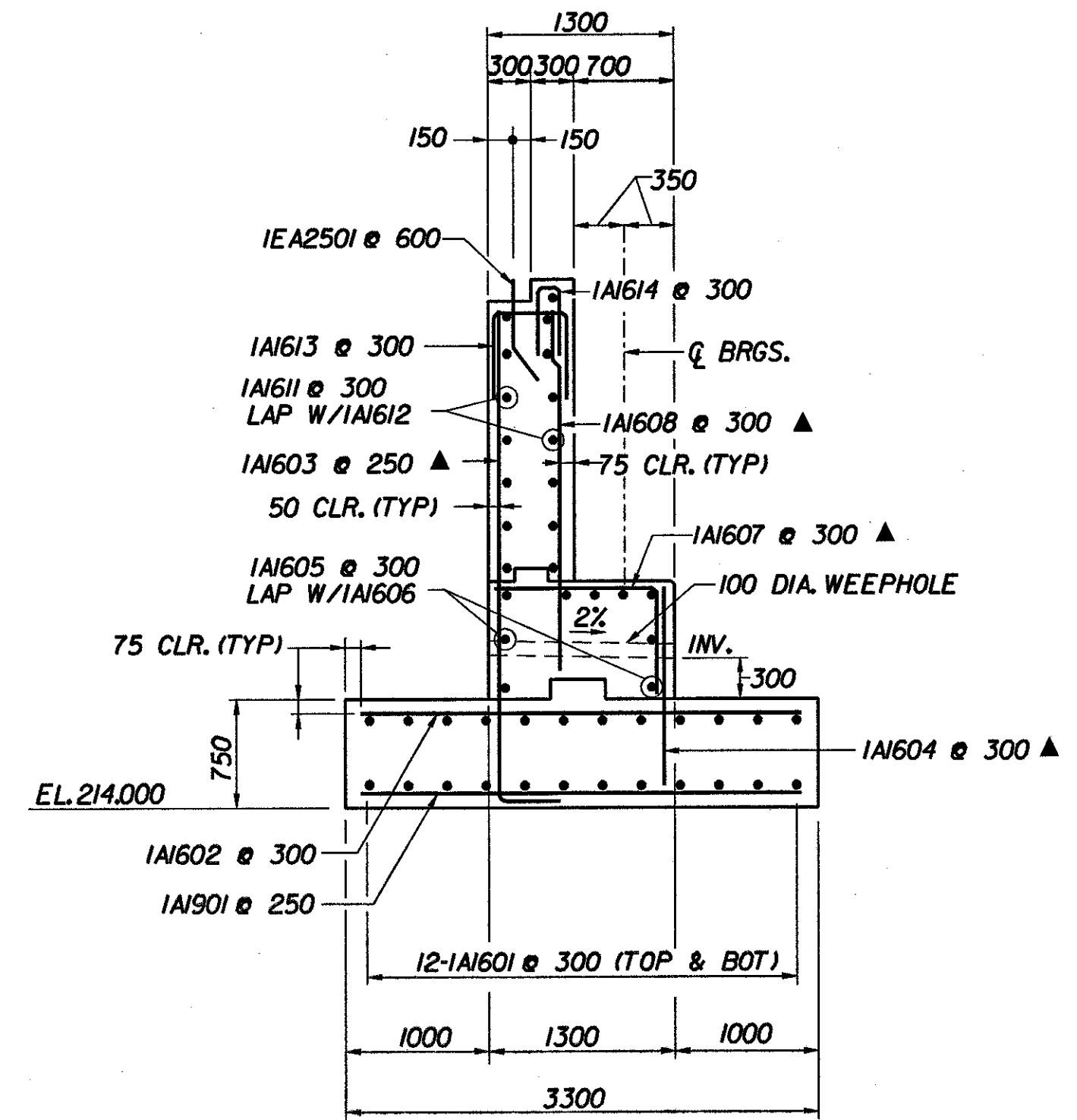
A ABUTMENT SECTION BR523 1:40 ASCT
