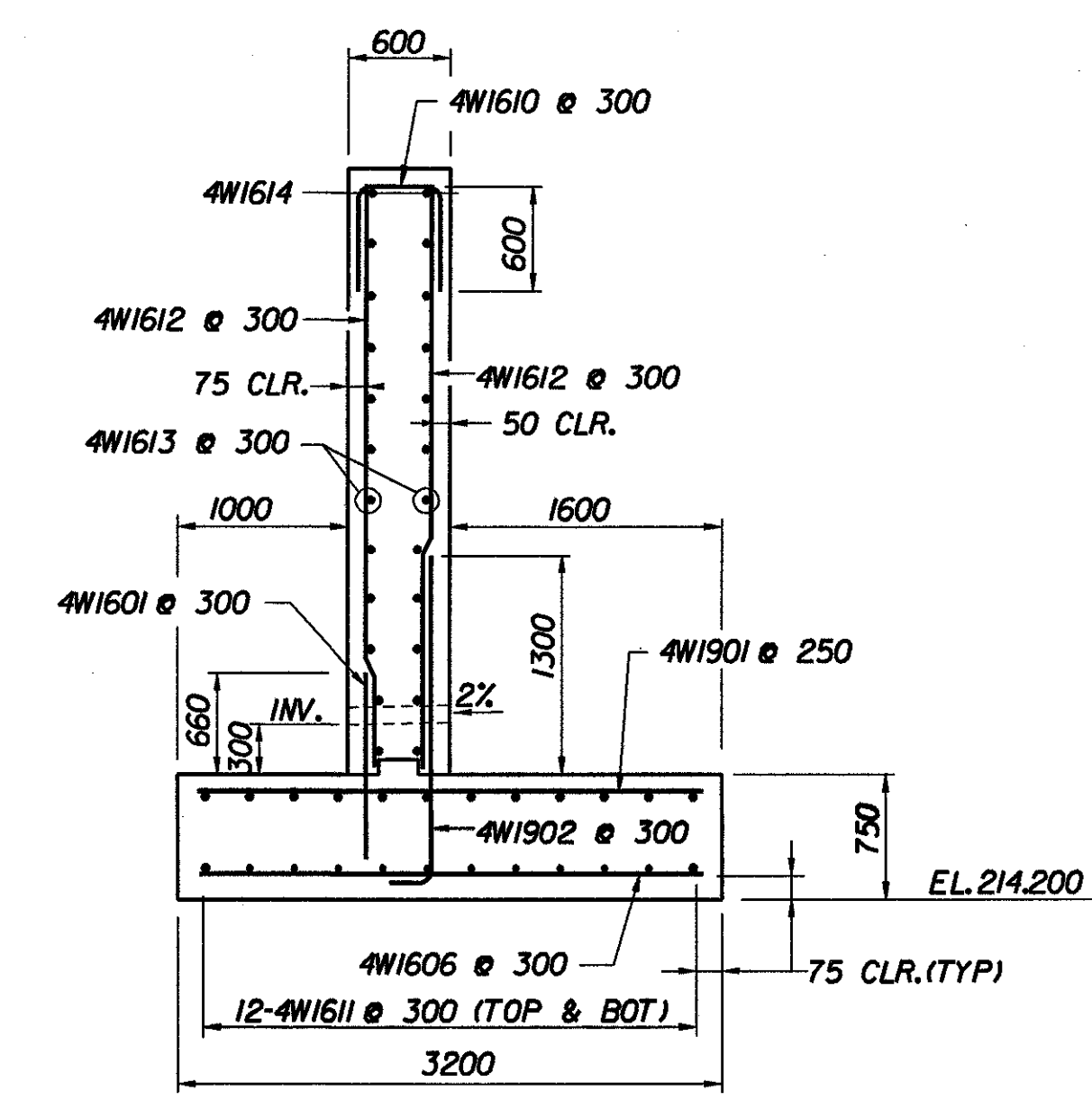
C WINGWALL 4 (LOW) SECTION BR430 1:40
