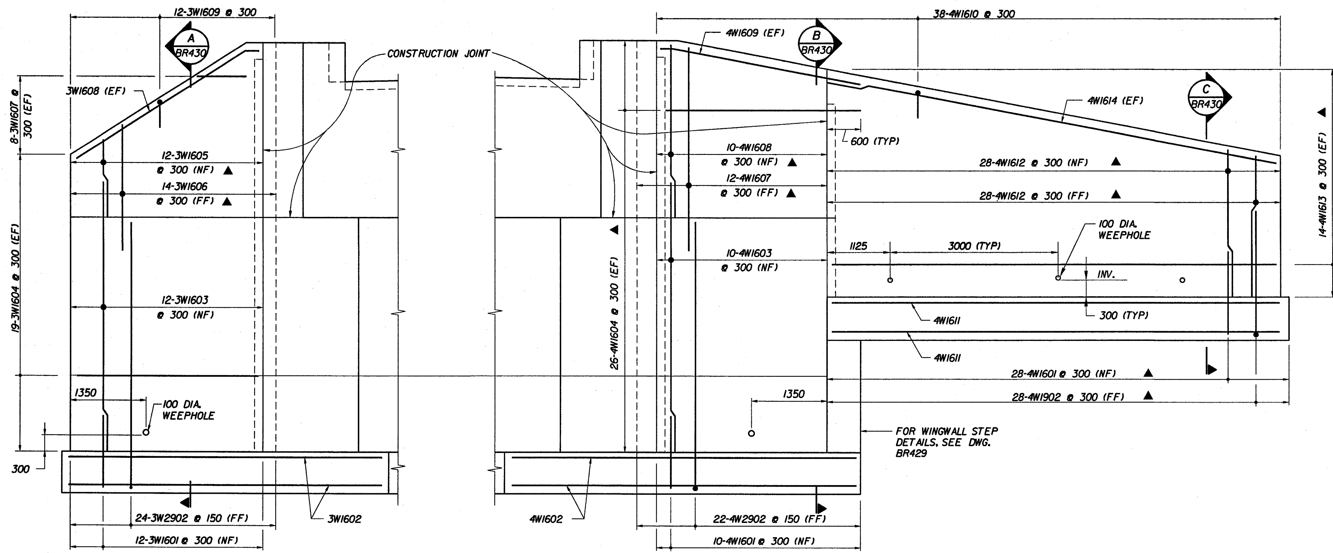
WINGWALL 3 ABUTMENT 2 WINGWALL REINFORCEMENT ELEVATIONS WINGWALL 4
