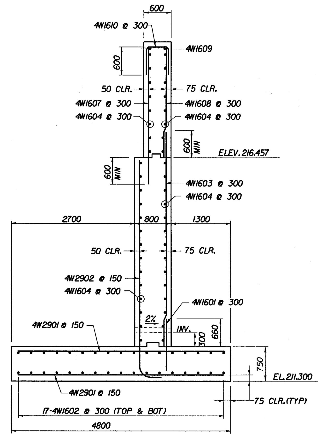
B WINGWALL 4 (HIGH) SECTION BR430 1:40
