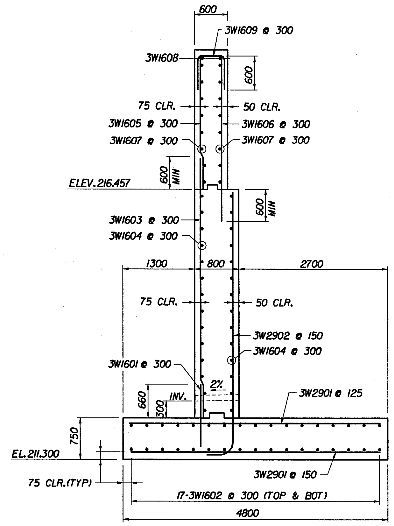
A WINGWALL 3 TYPICAL SECTION BR430 1:40
