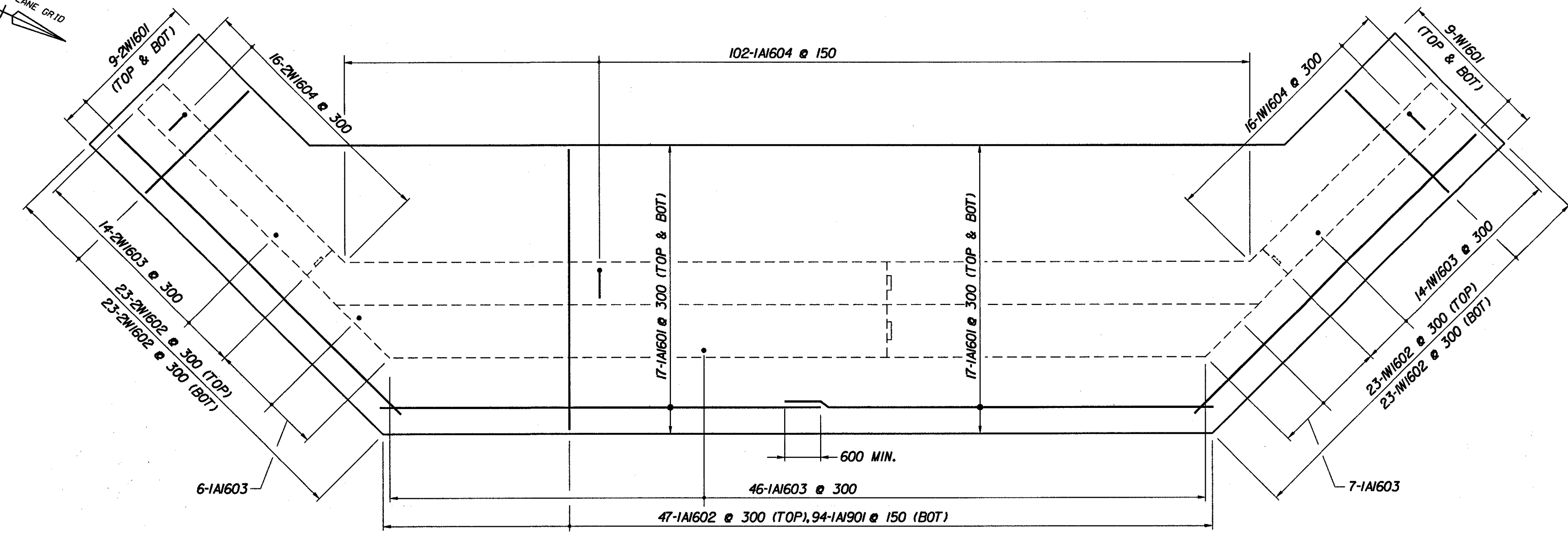
ABUTMENT 1 FOOTING REINFORCEMENT PLAN
