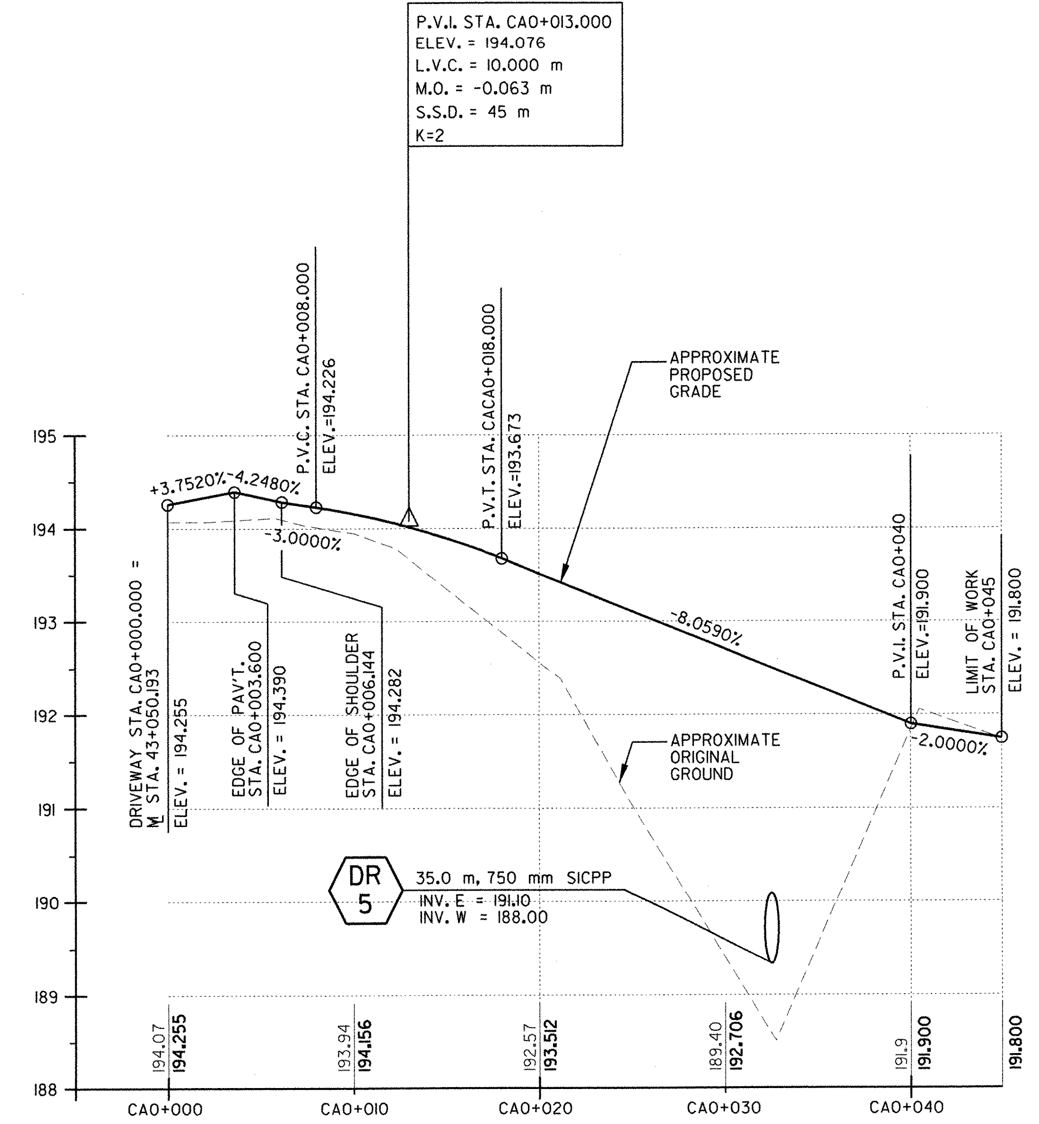
DRIVEWAY 5 1:200 1:40 PROFILE
