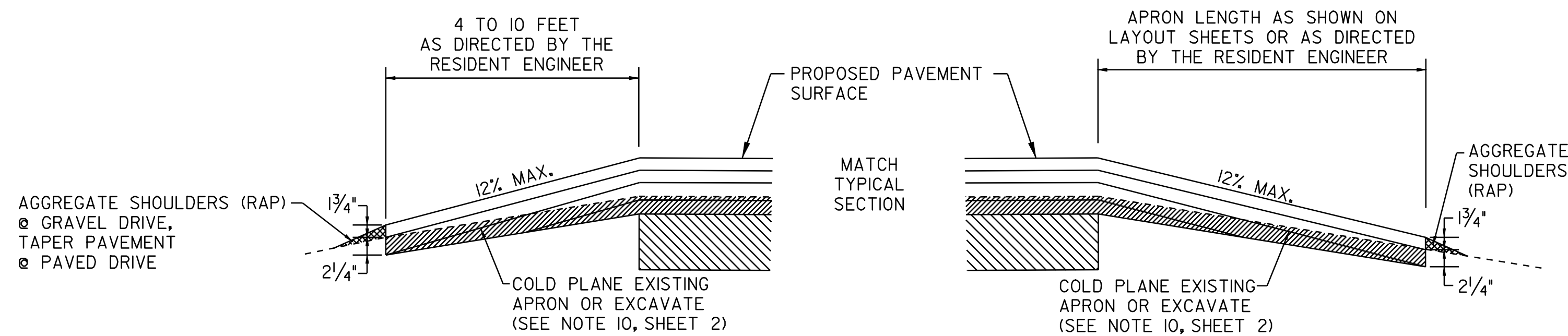
TOWN HIGHWAY TRANSITION DETAIL @ COLD PLANE/RECLAIM AREAS
