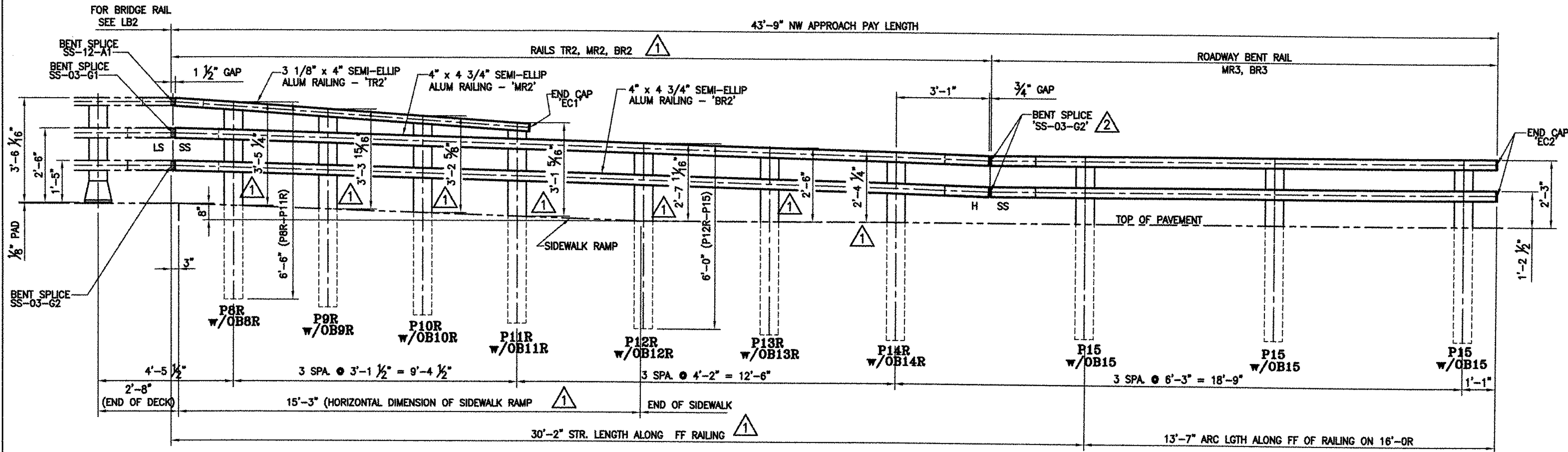
INSIDE ELEVATION OF NW SIDEWALK APPROACH RAIL (STA.18+30 LT. - STA.100+55 LT.)
