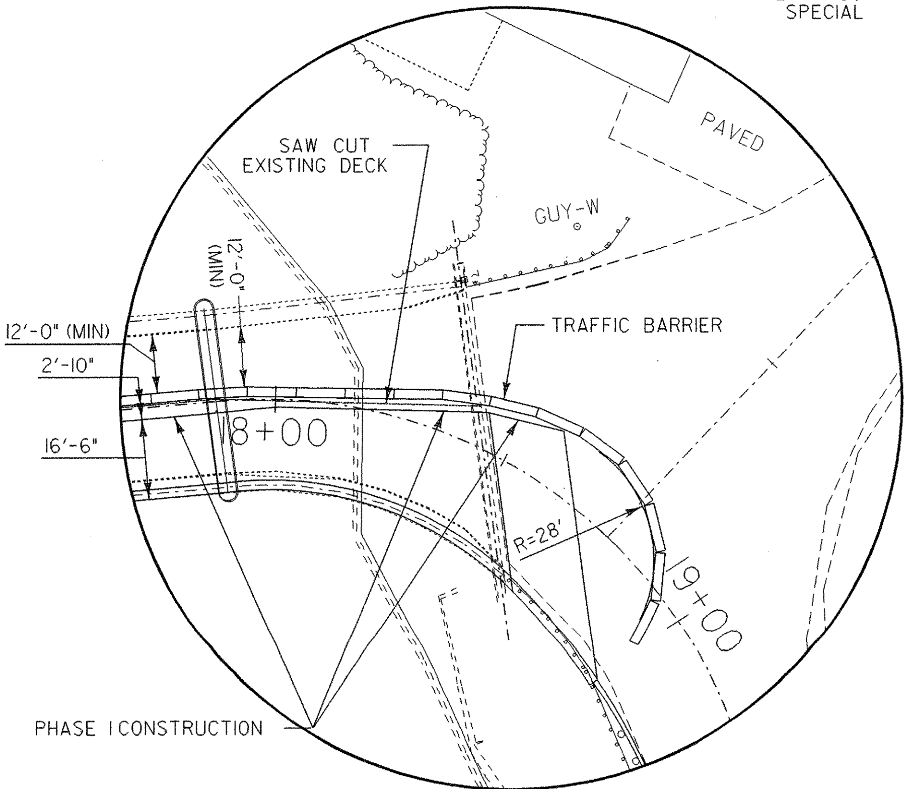
DETAIL "B" SCALE: 1"=20'
