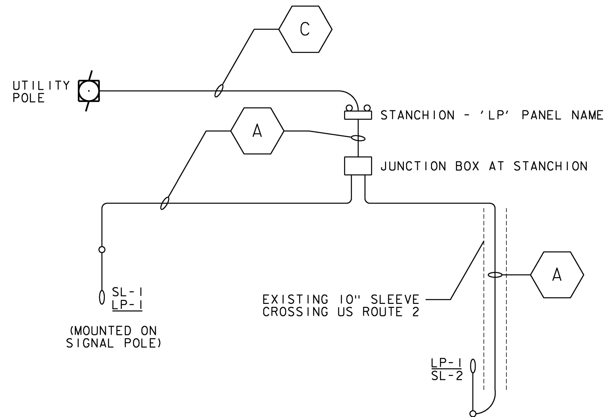
ONE-LINE DIAGRAM NOT TO SCALE
