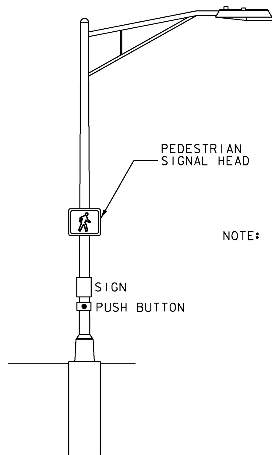
STREET LIGHT WITH PEDESTRIAN SIGNAL DETAIL NOT TO SCALE
