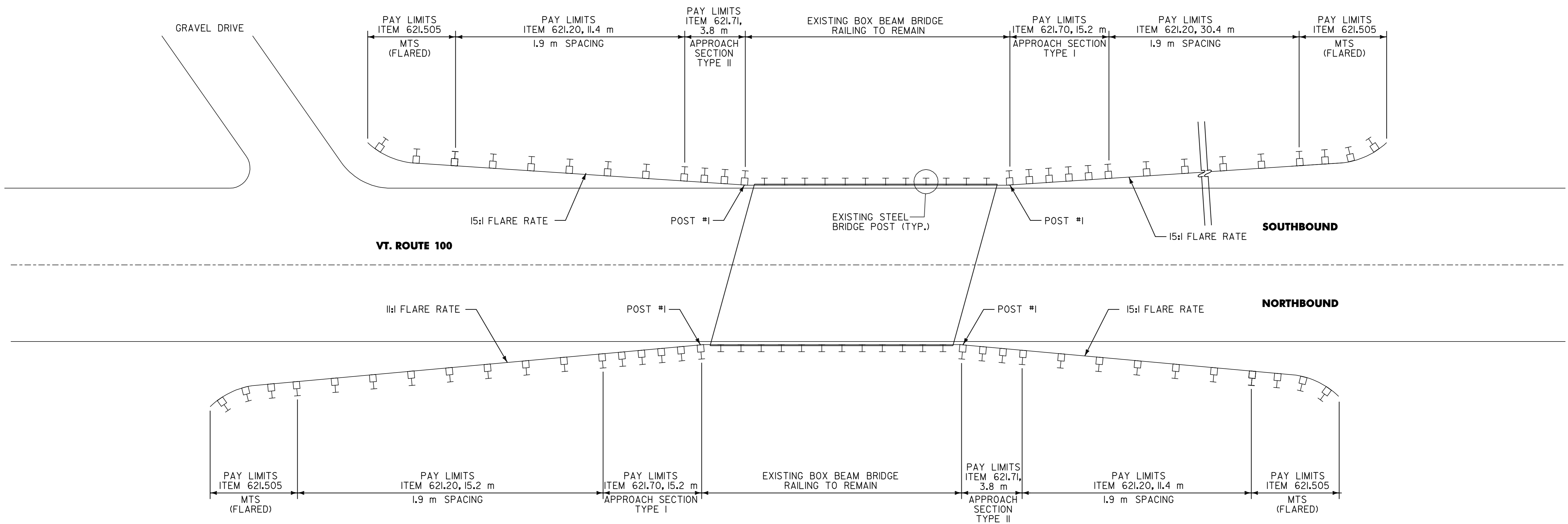
BR 147 GRANVILLE MM 0.422 = STA. 0+679.143 NOT TO SCALE
