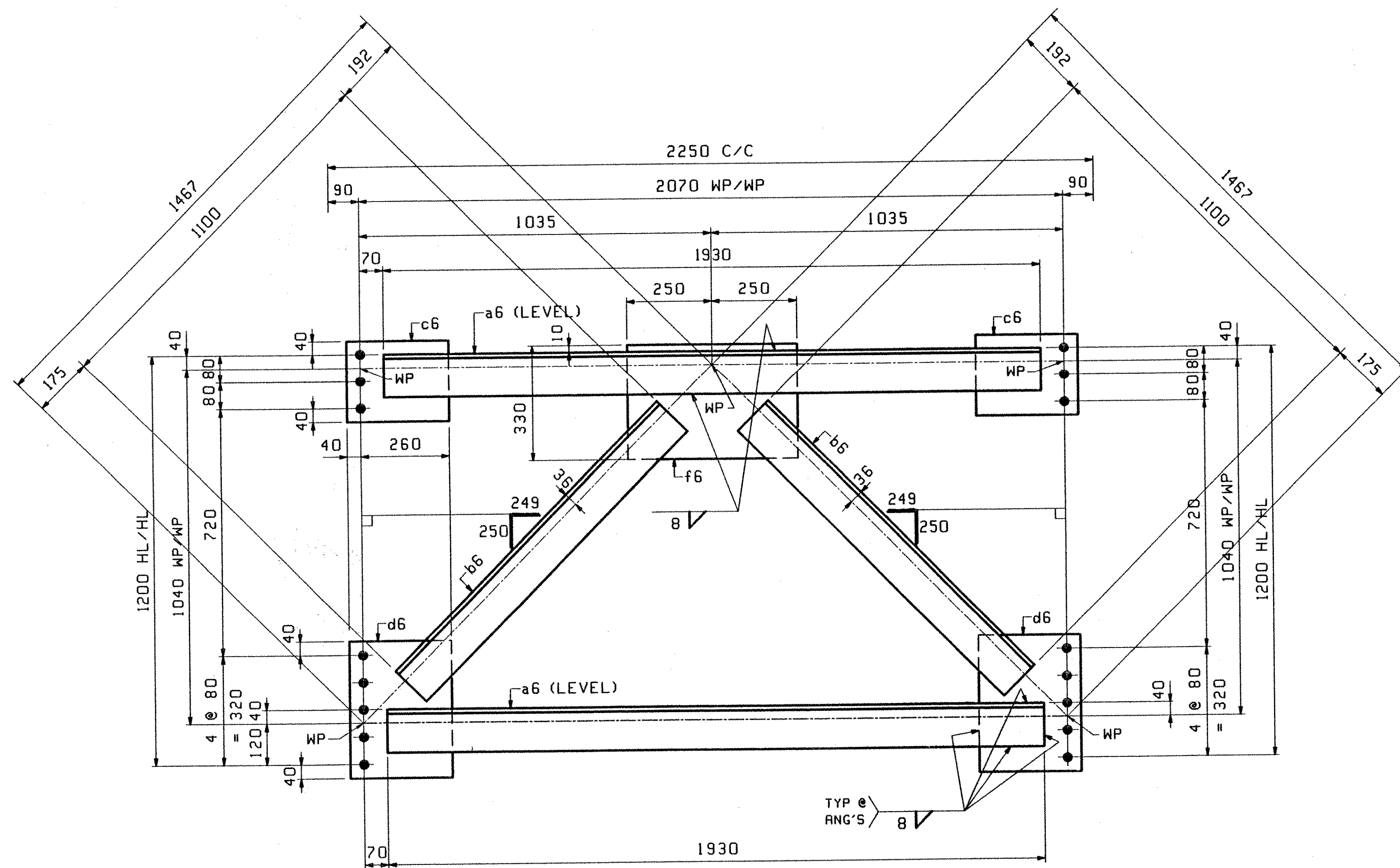
20 ~ INTERMEDIATE CROSSFRAMES ~ 6CF1
