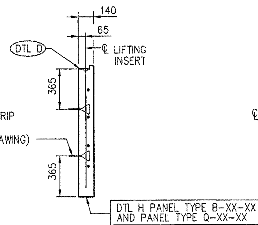
SECTION B-B SECTION C-C SCALE 1:20
