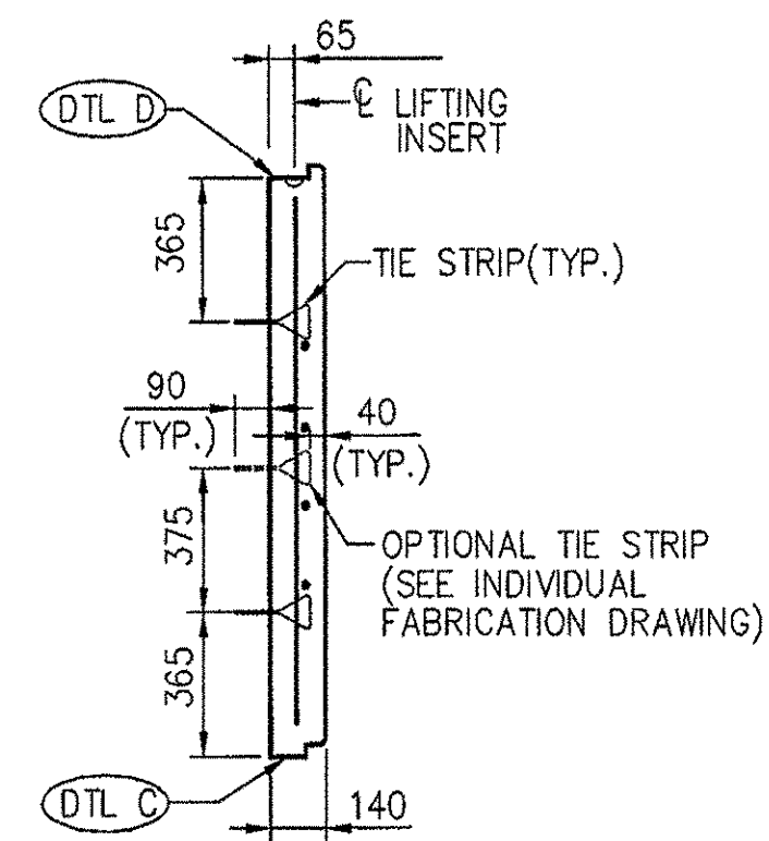
SECTION B-B SECTION C-C SCALE 1:20
