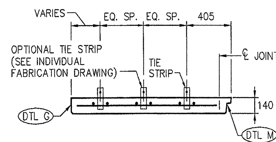
SECTION K-K SCALE 1:20
