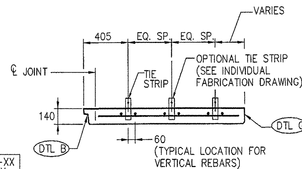
SECTION L-L SCALE 1:20
