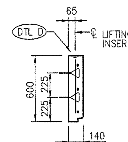
SECTION S-S SCALE 1:20
