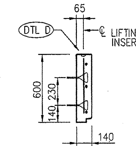
SECTION U-U SCALE 1:20
