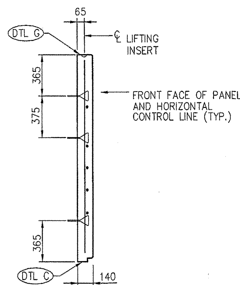
SECTION J-J SCALE 1:20
