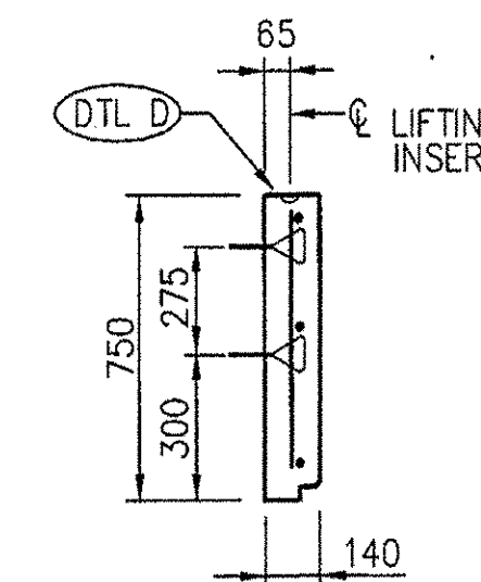
SECTION T-T SCALE 1:20
