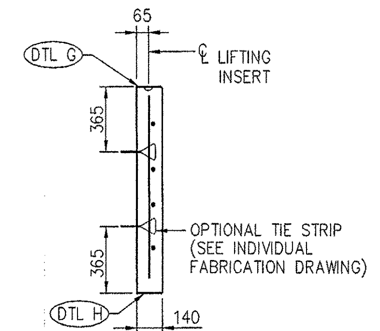
SECTION H-H SCALE 1:20
