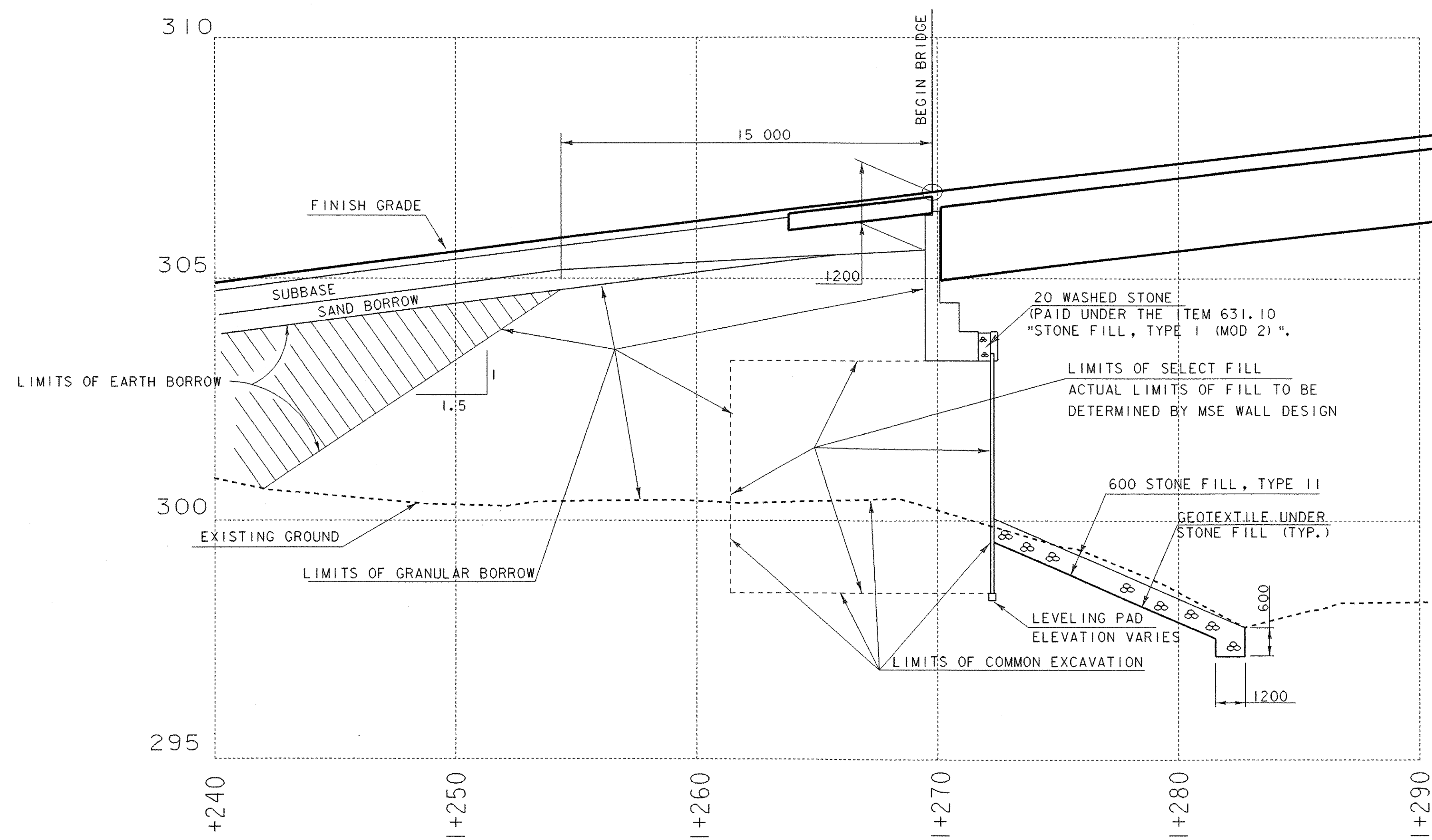
ABUTMENT I EARTH WORK TYPICAL SECTION
