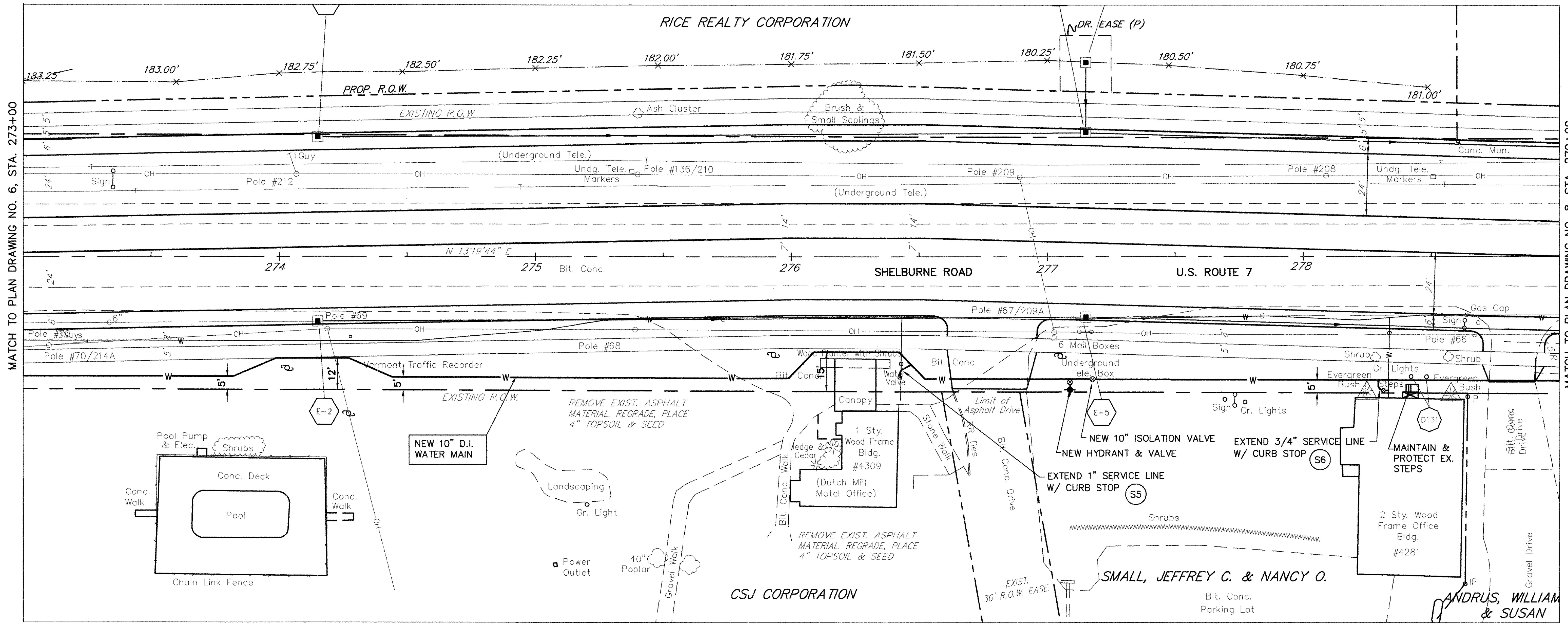
PLAN 1" = 20'
