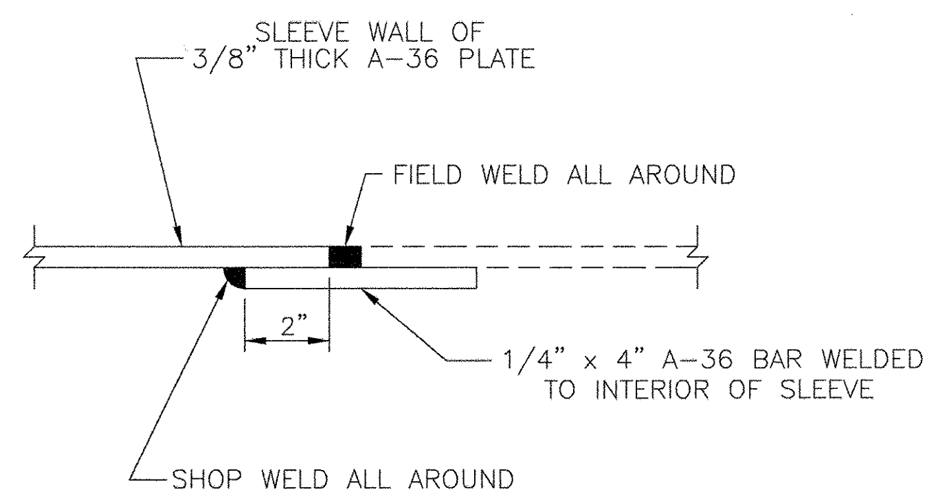
STEEL SLEEVE ENCASEMENT JOINT WELD DETAIL
