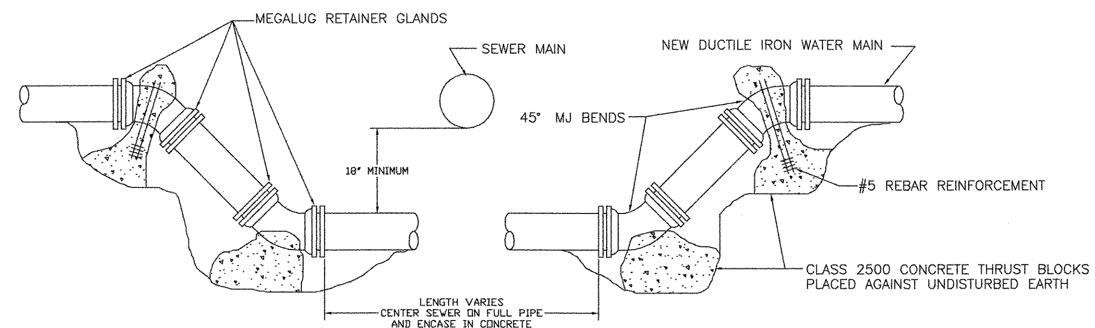
WATERLINE CROSSING SEWER LINE DETAIL
