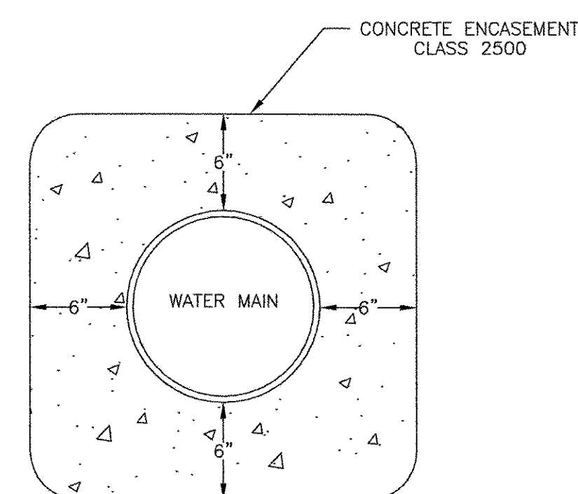
WATER LINE CONCRETE ENCASEMENT DETAIL
