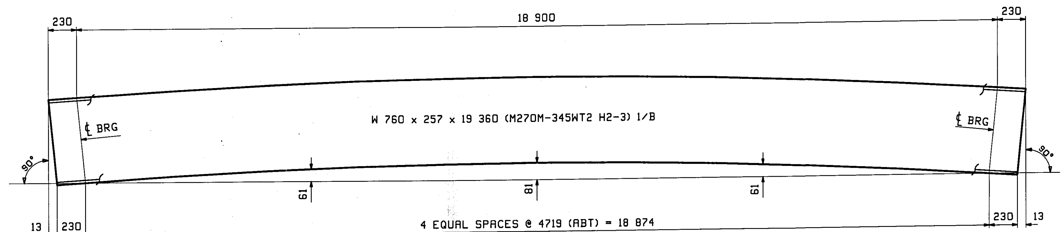
CAMBER DIAGRAM FOR 1S1,2S2,2S3,3S4 & 1S5
