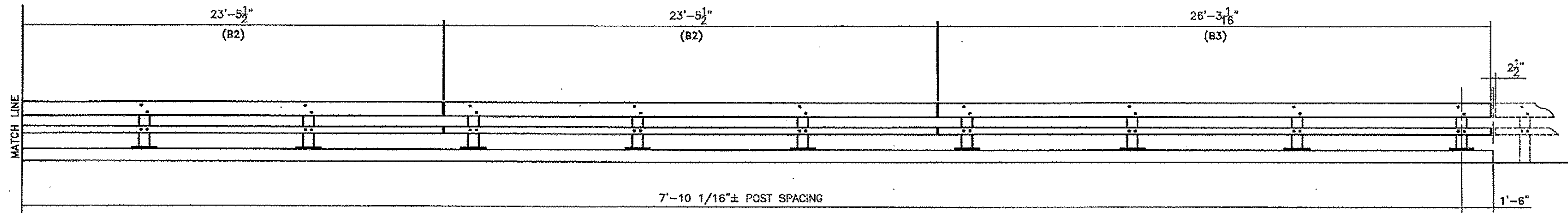
TYPICAL RAIL ELEVATION looking from center of road
