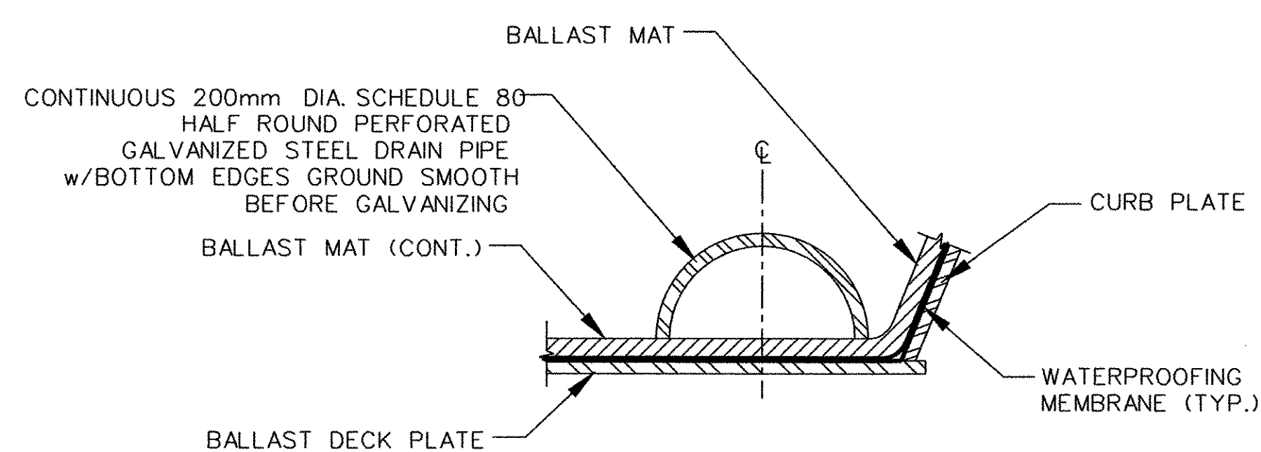
DRAIN PIPE DETAIL
