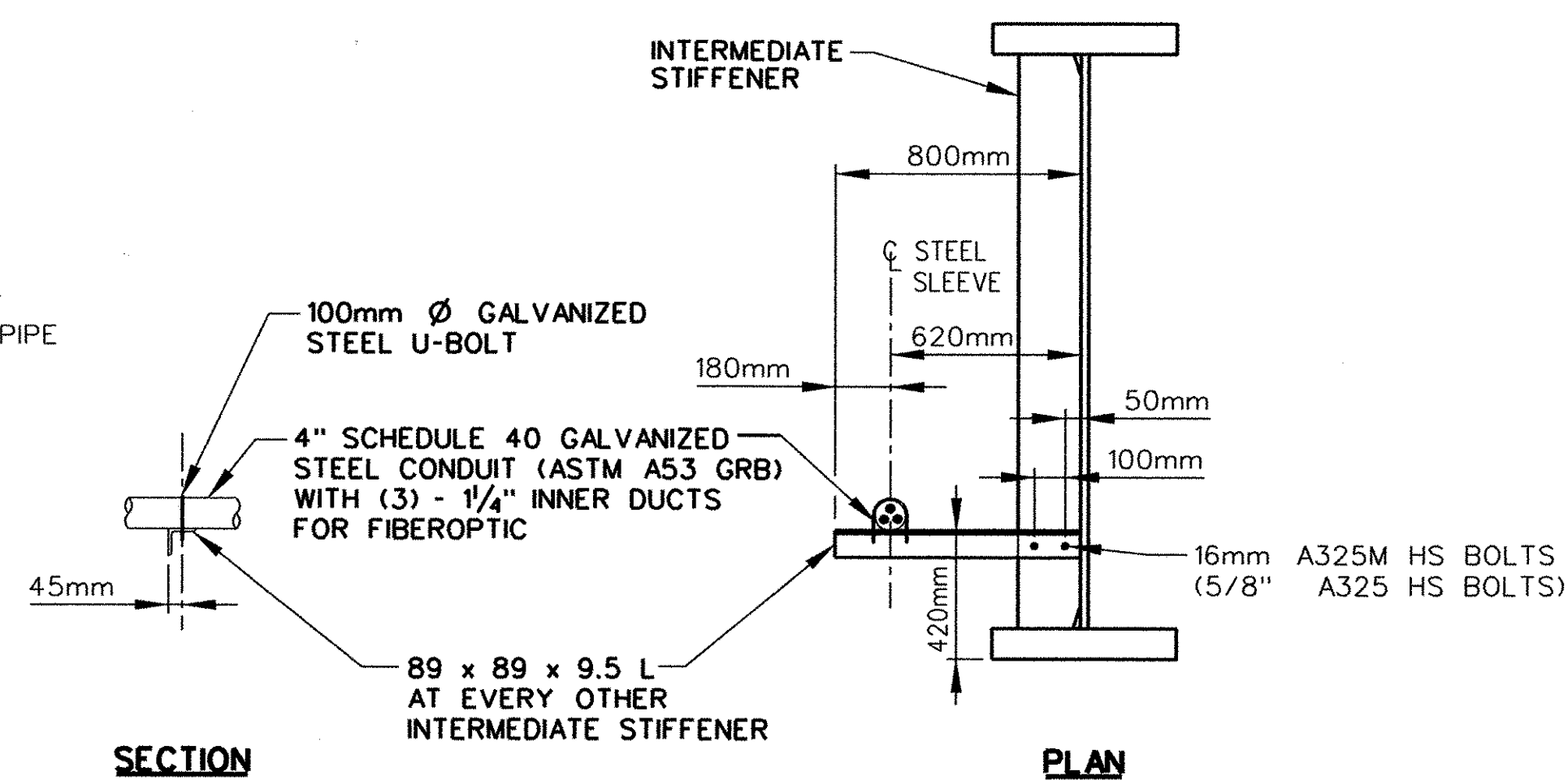
FIBEROPTIC CONDUIT SUPPORT DETAIL
