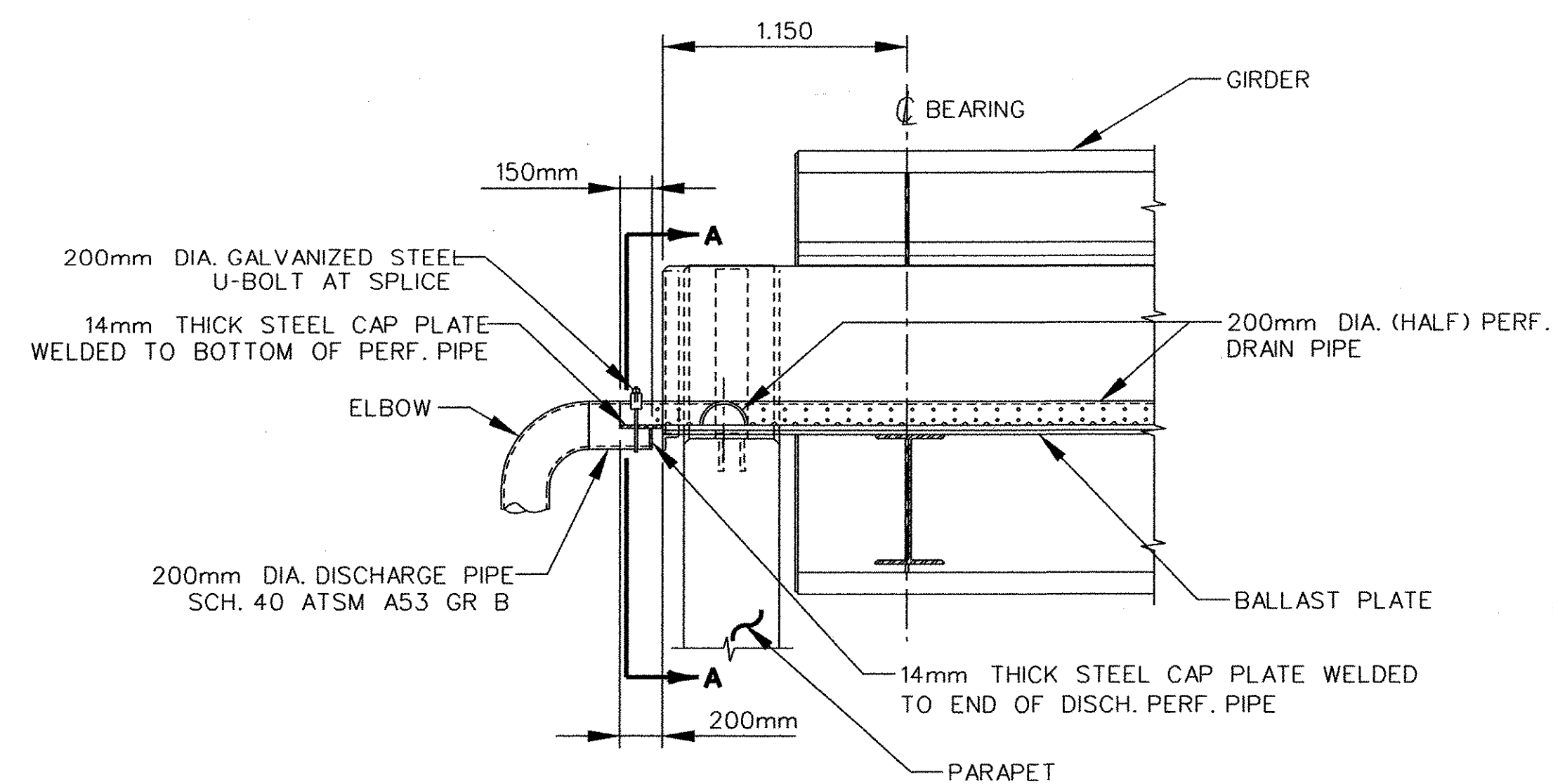
PARAPET DISCHARGE PIPE CONNECTION DETAIL
