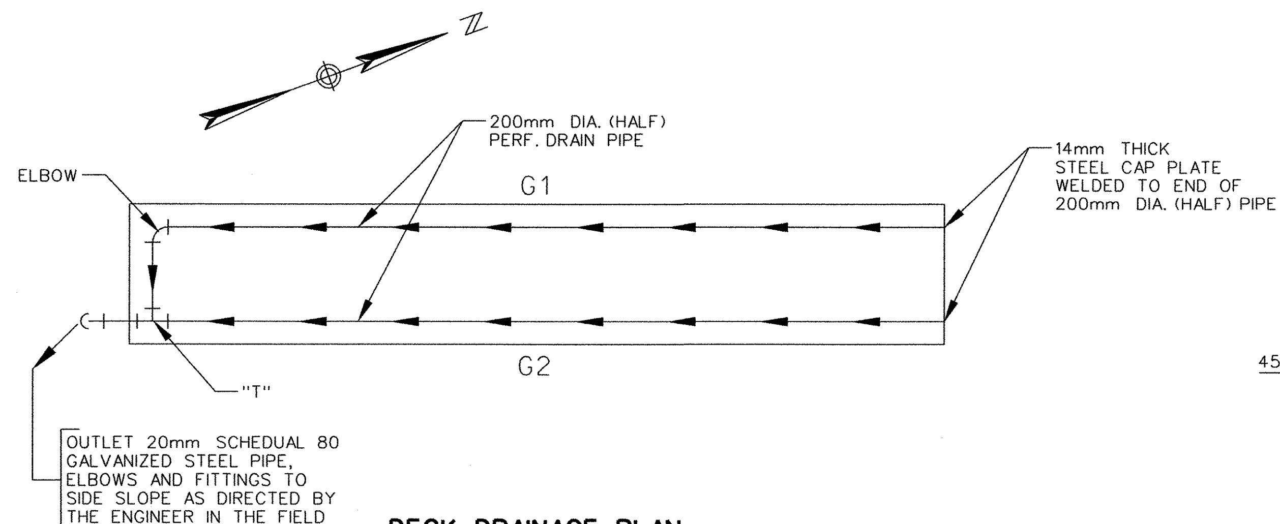
DECK DRAINAGE PLAN
