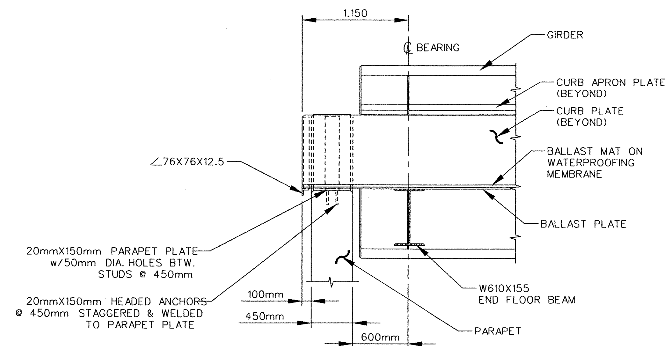
PARAPET DETAIL
