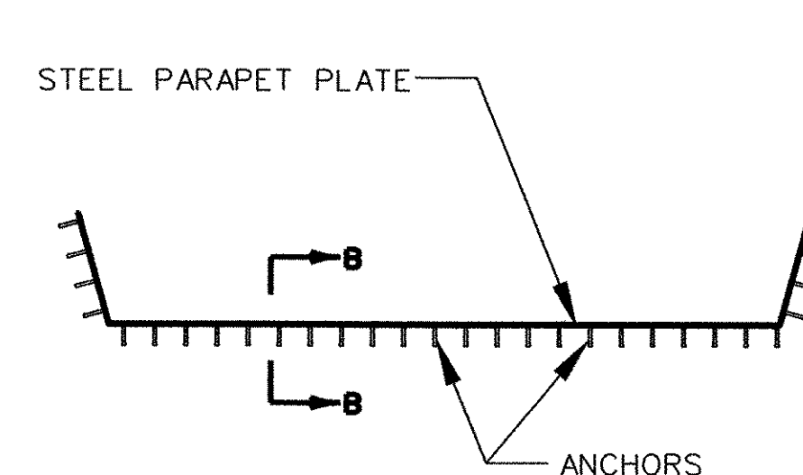
PARAPET PLATE DETAIL
