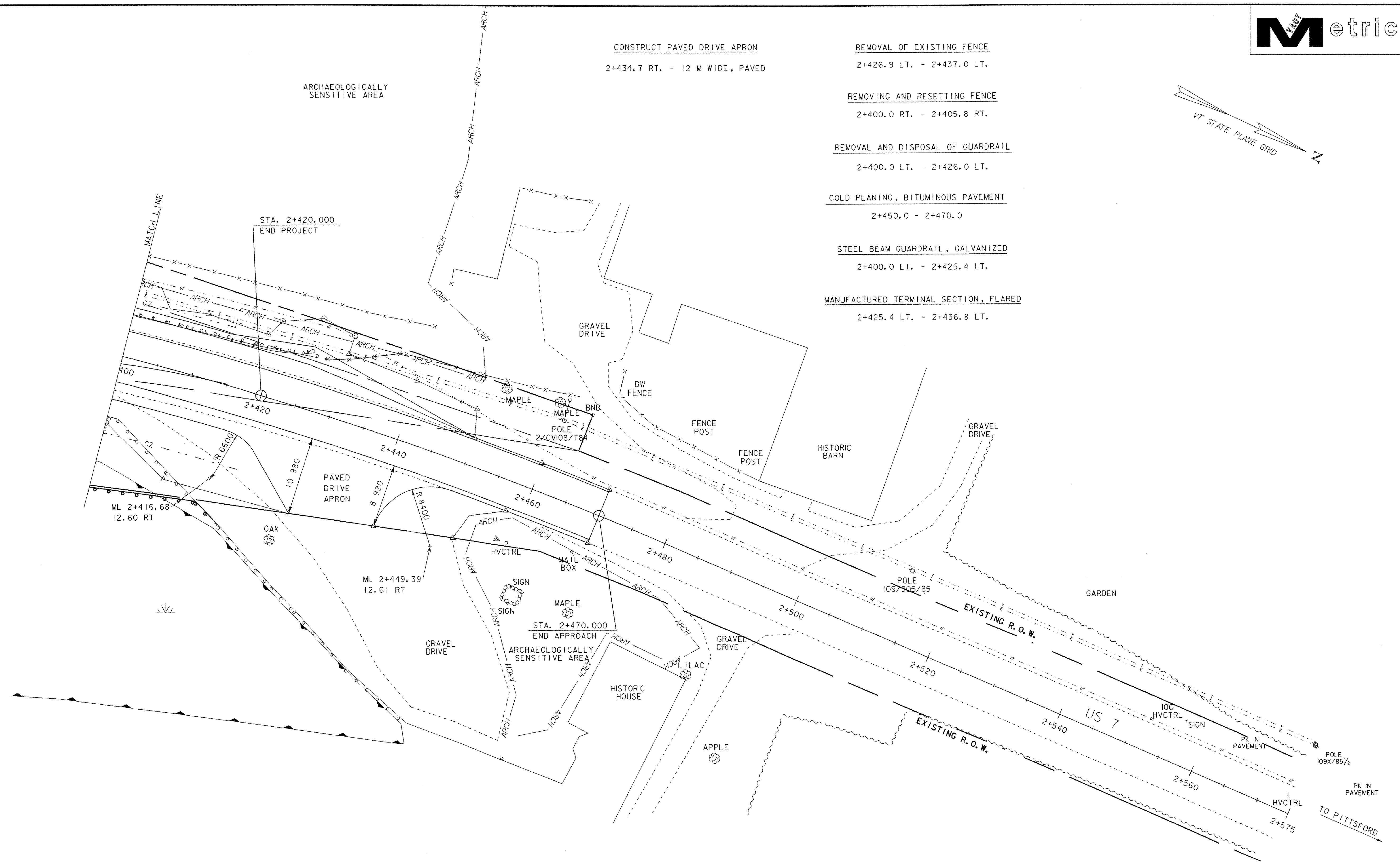
LAYOUT PLAN 3
