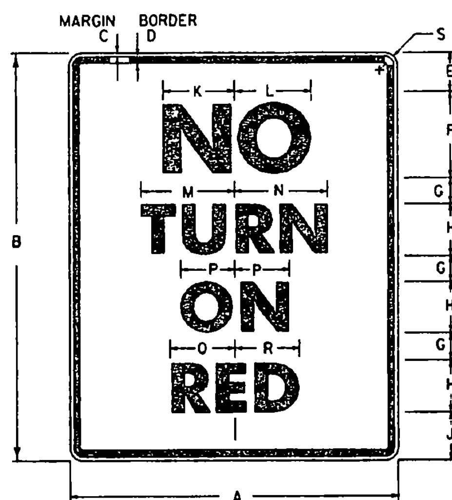
POST MOUNTING R10-11A
