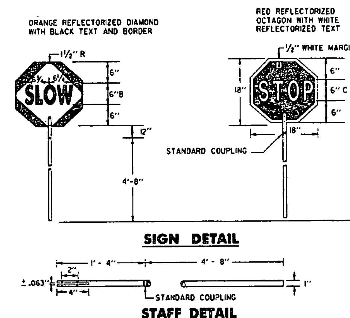
STAFF DETAIL
