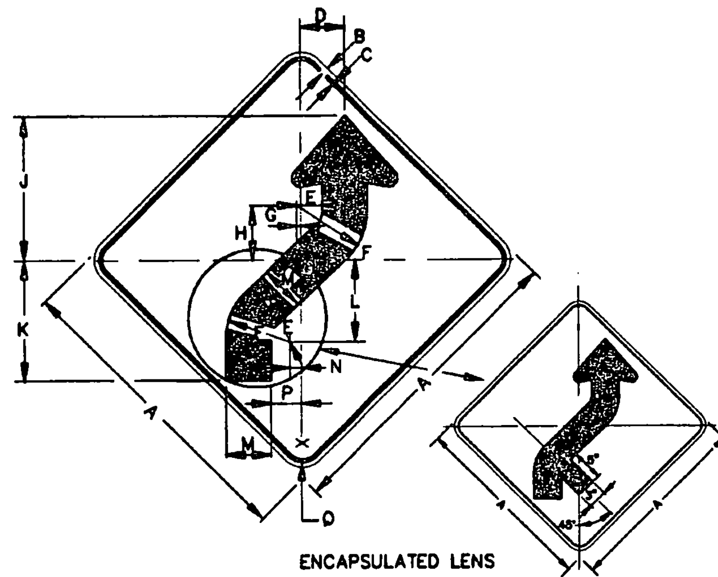
ENCAPSULATED LENS
