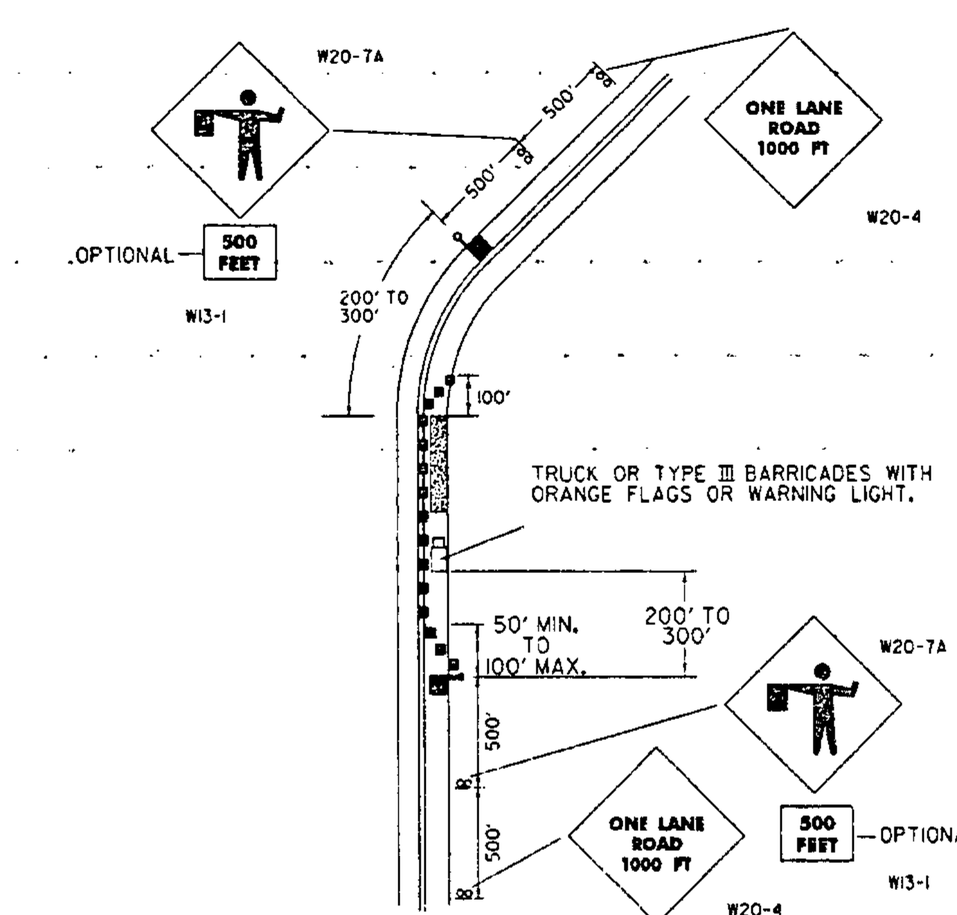
TYPICAL APPLICATIONS - DAYTIME MAINTENANCE OPERATIONS OF SHORT DURATION ON A 2-LANE ROADWAY WHERE FLAGGING IS PROVIDED
