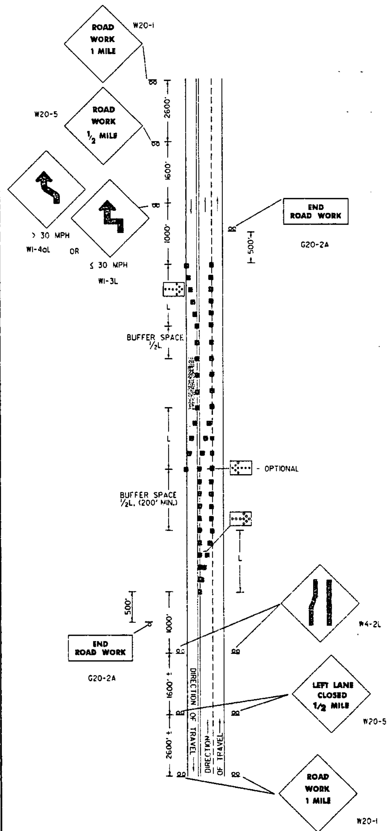
TYPICAL APPLICATION - DAYTIME MAINTENANCE OPERATION OF SHORT DURATION ON A 3 LANE ROADWAY WHERE CENTER LANE IS USED FOR OPPOSING TRAFFIC
