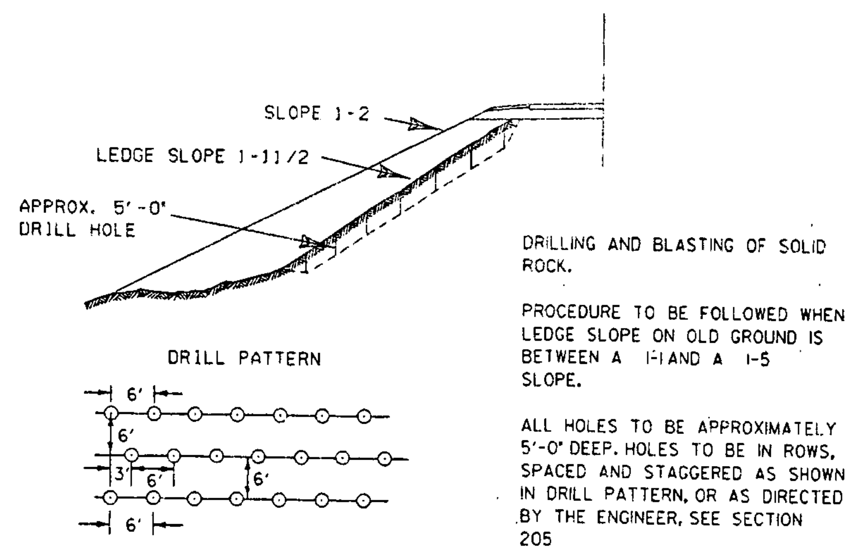
TYPICAL NEAT PAY LINES FOR MUCK EXCAVATION
