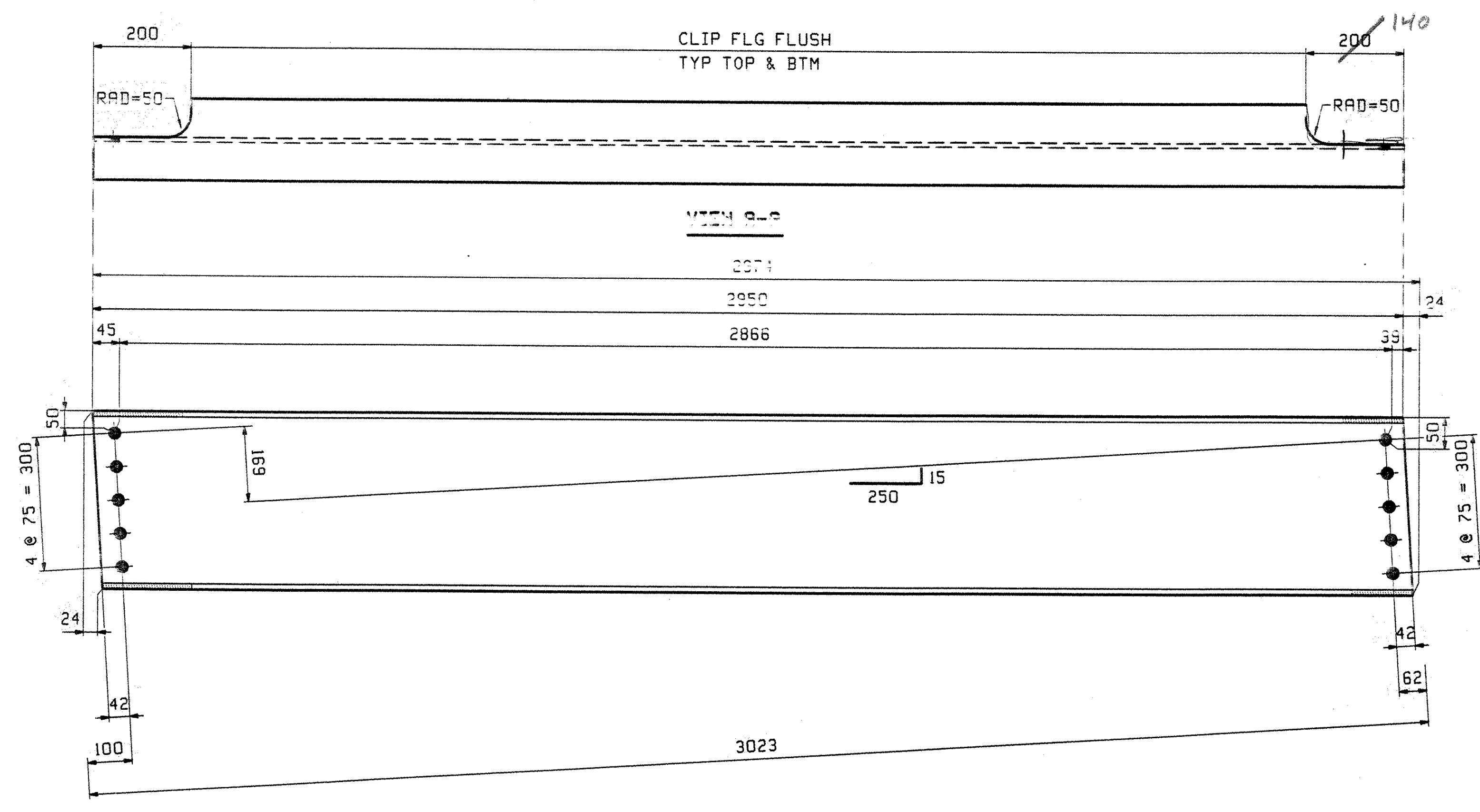
1 - END DIAPHRAGM - 13D1
