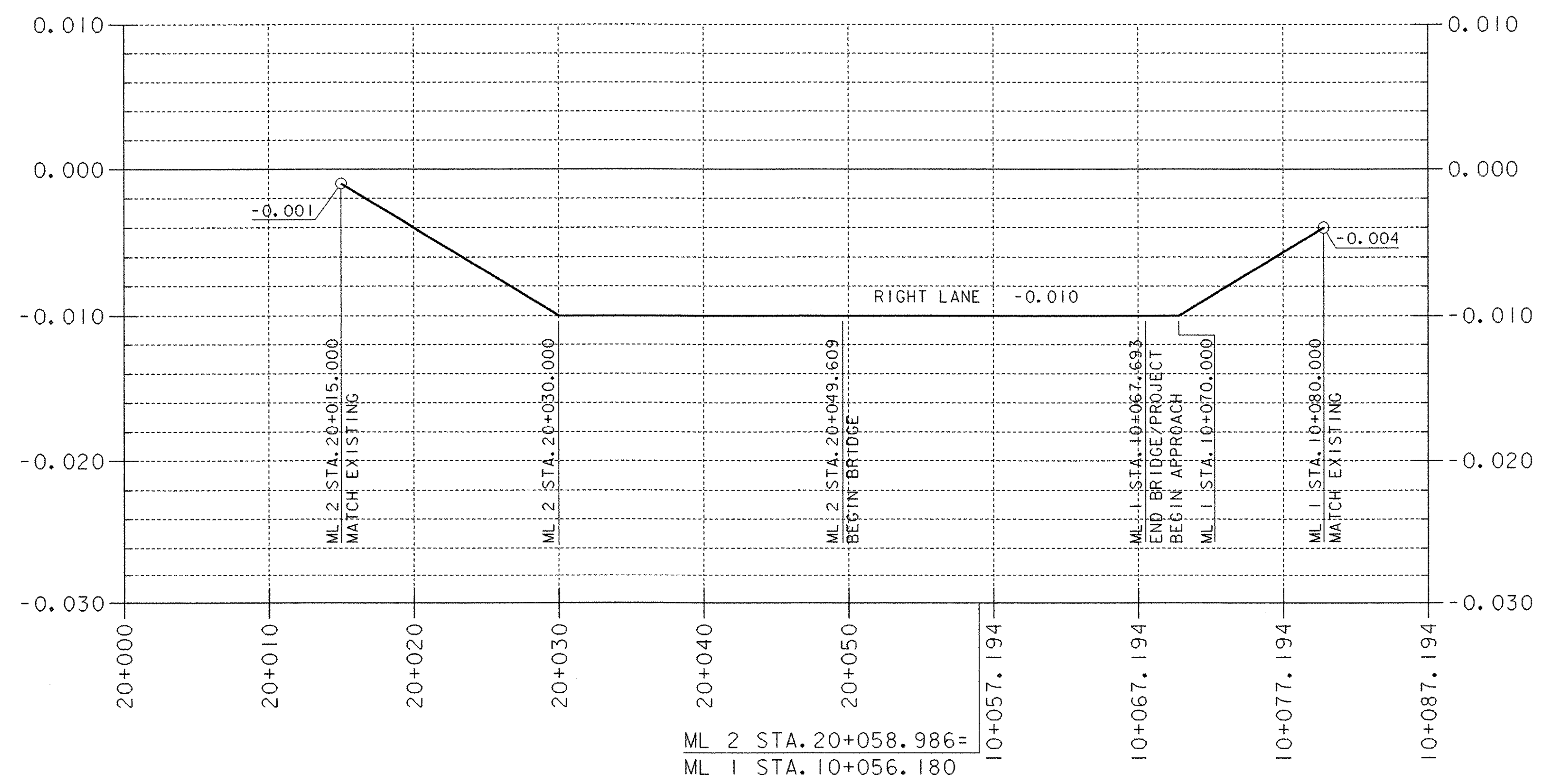
Banking Diagram For Right Travel Lane - Bridge St. to Main St.
