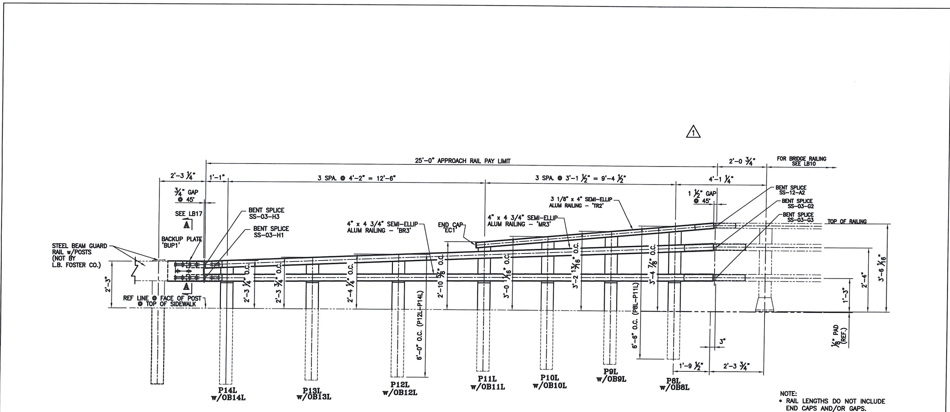
INSIDE ELEVATION OF NY APPROACH RAIL (FOR NE APPROACH SEE LB12A)
