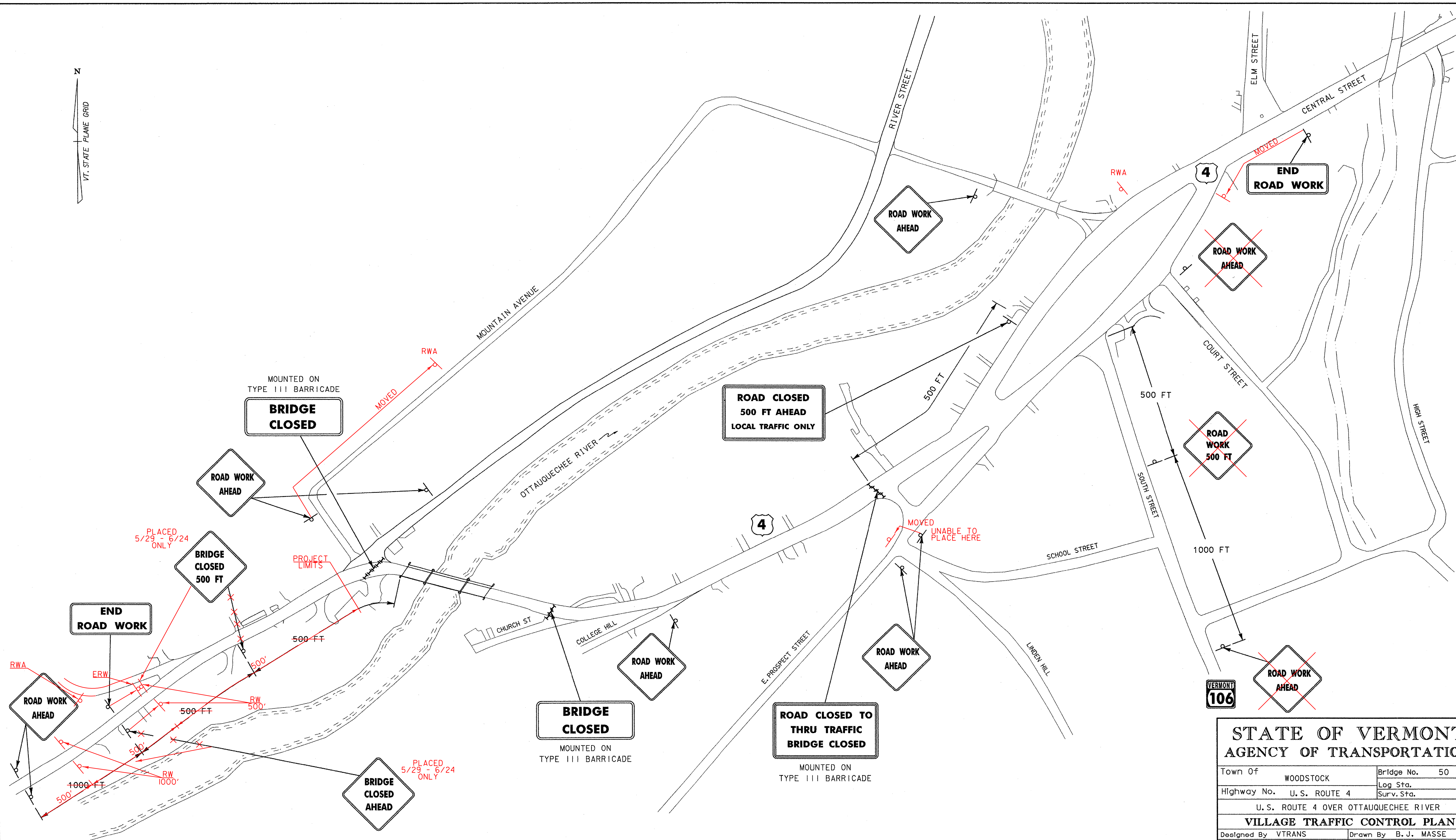
VILLAGE TRAFFIC CONTROL PLAN SCALE: 1" = 200'
