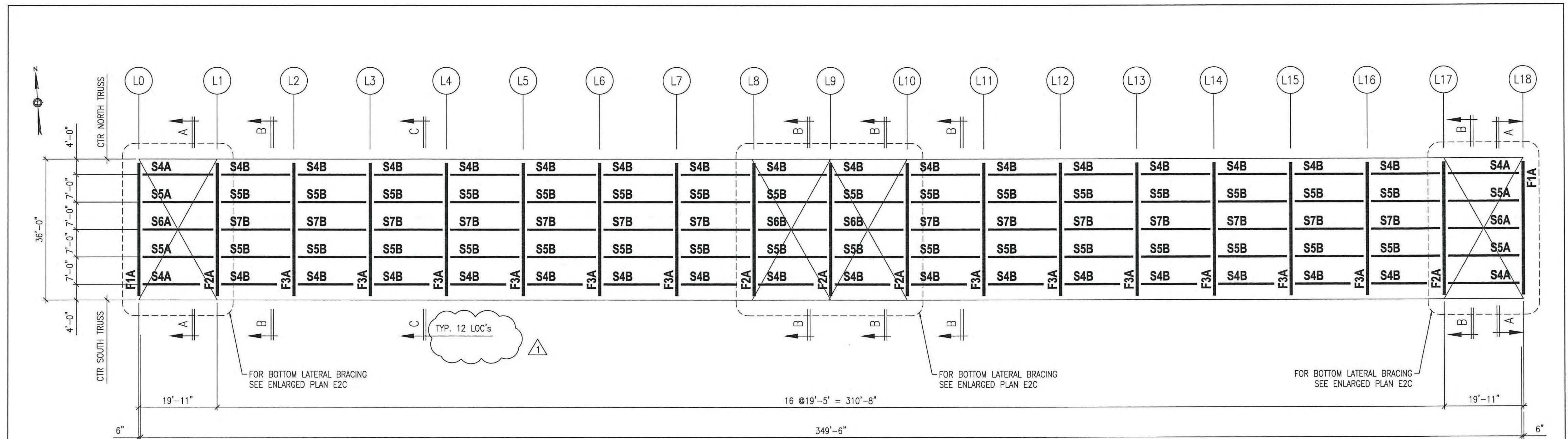
STRINGER & FLOOR BEAM PLAN
