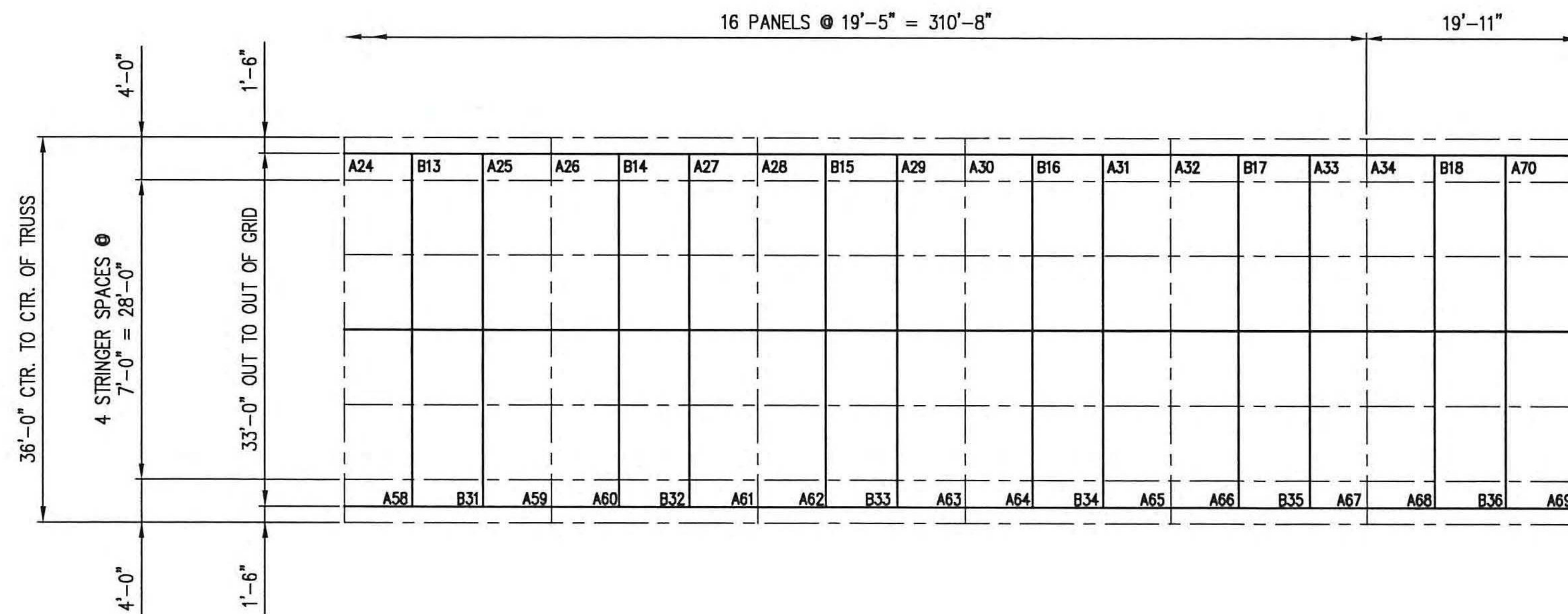
PLAN VIEW
