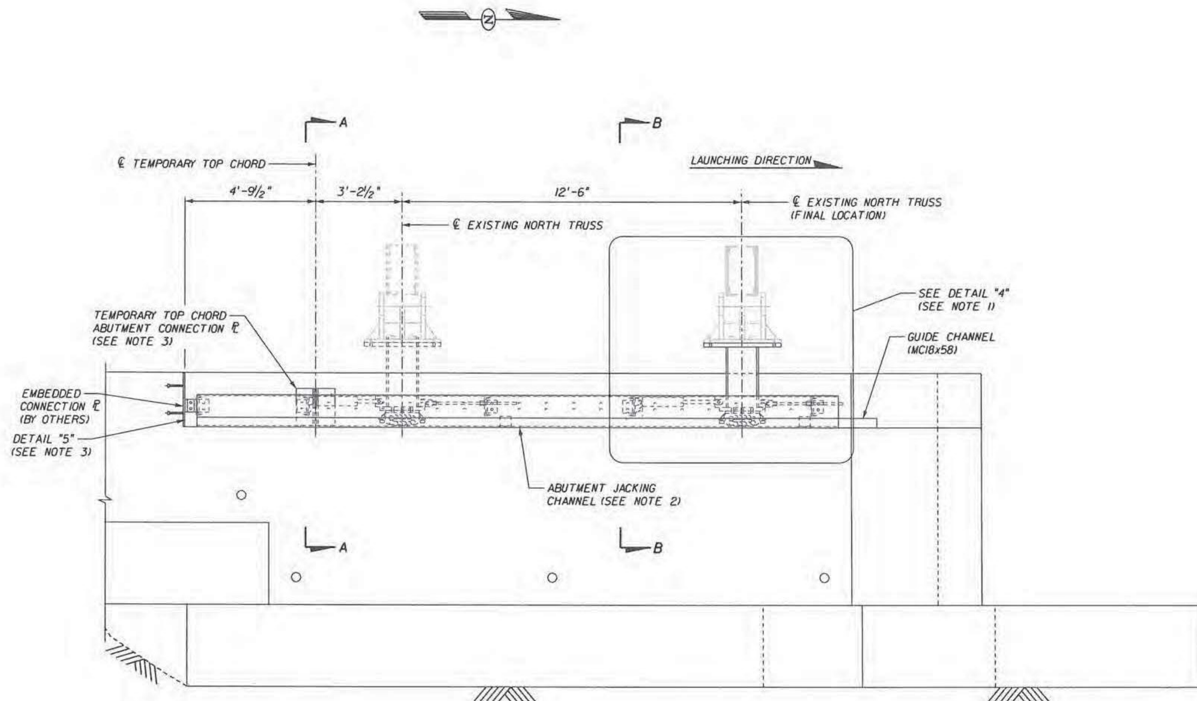
ABUTMENT TYPICAL SECTION (WEST ABUTMENT SHOWN, EAST ABUTMENT SIMILAR) (LOOKING DOWNSTATION)
