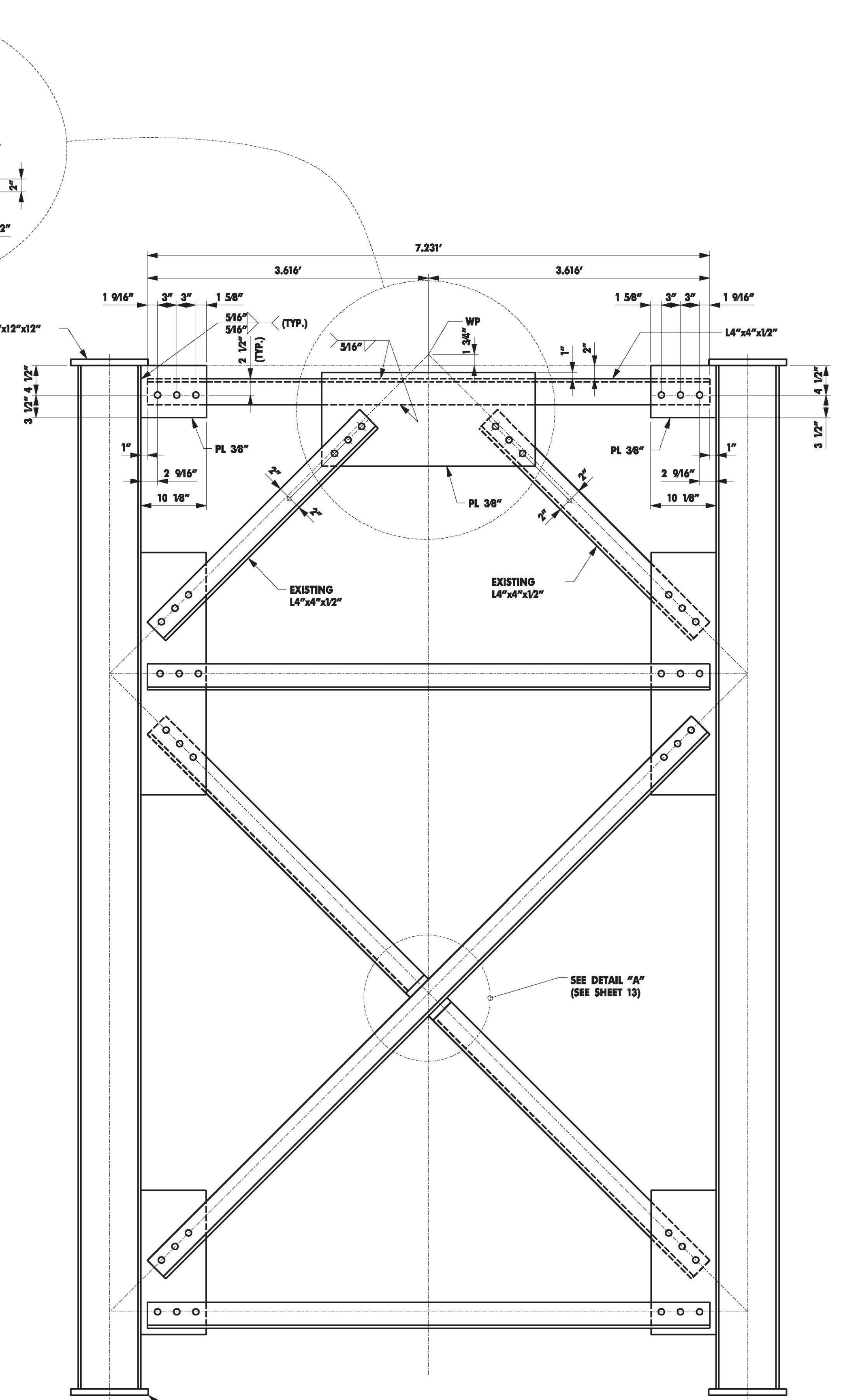
SECTION N-N
