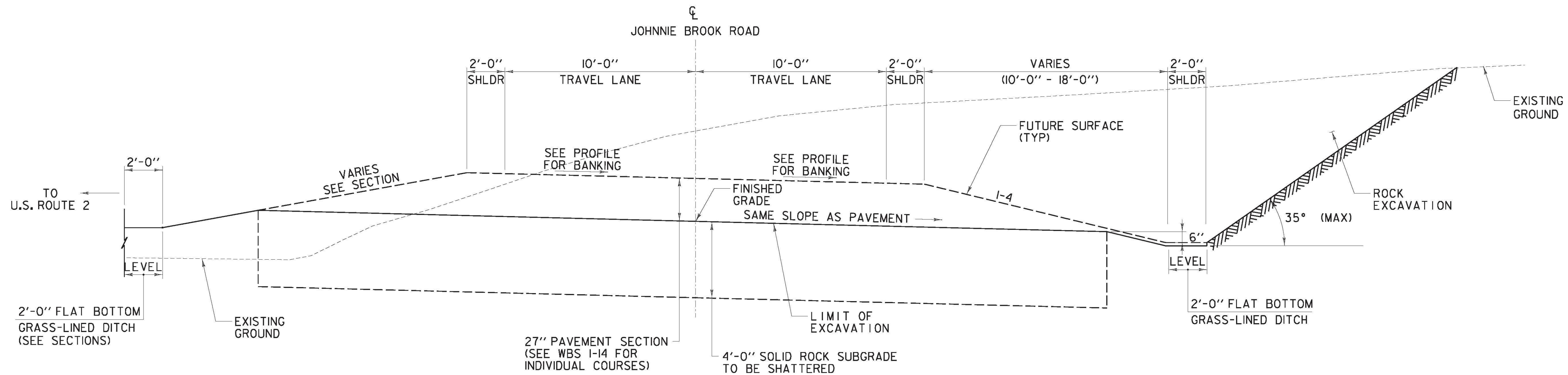
JOHNNIE BROOK ROAD TYPICAL SECTION STA JB 120+75.00 TO STA JB 123+75.00
