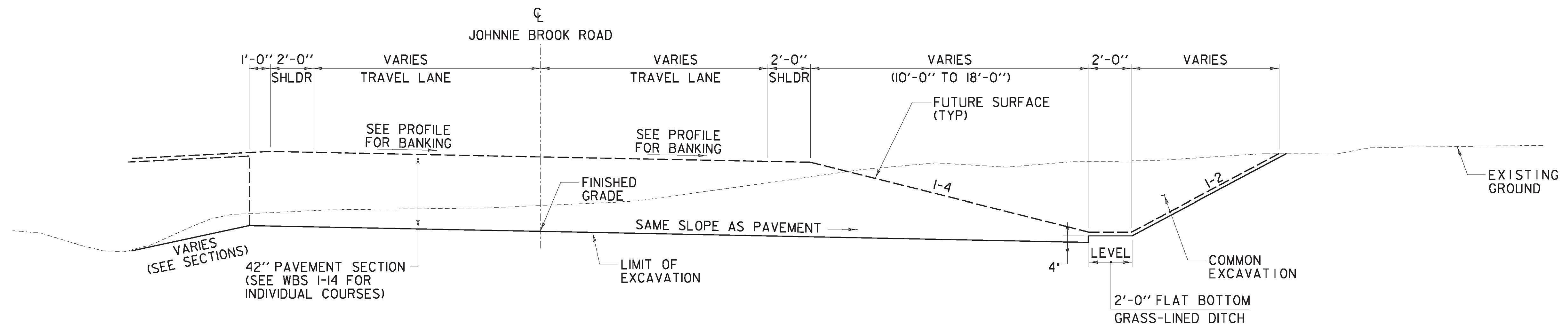
JOHNNIE BROOK ROAD TYPICAL SECTION STA JB 120+12.00 TO STA JB 120+75.00
