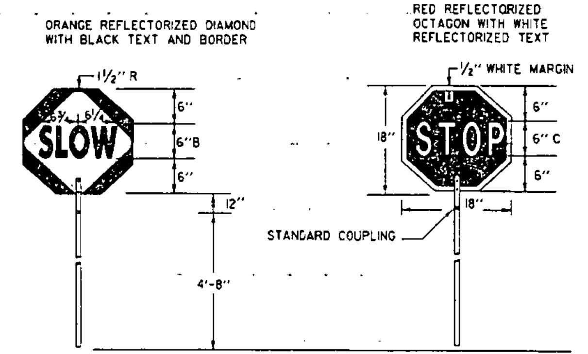
SIGN DETAIL
