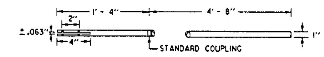
STAFF DETAIL
