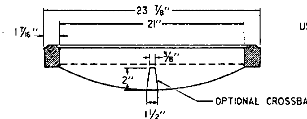
SECTION B-B
