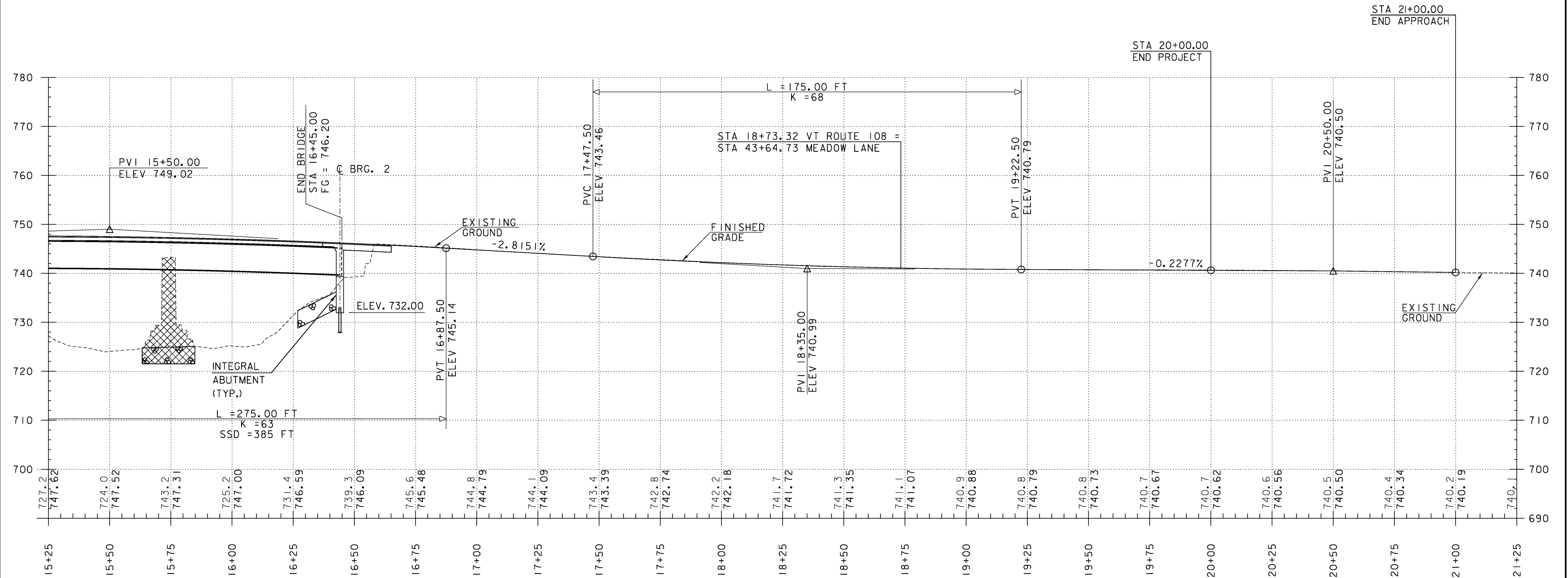
PROFILE VT 108 HOR. SCALE 1" = 20'-0" VER. SCALE 1" = 10'-0"
