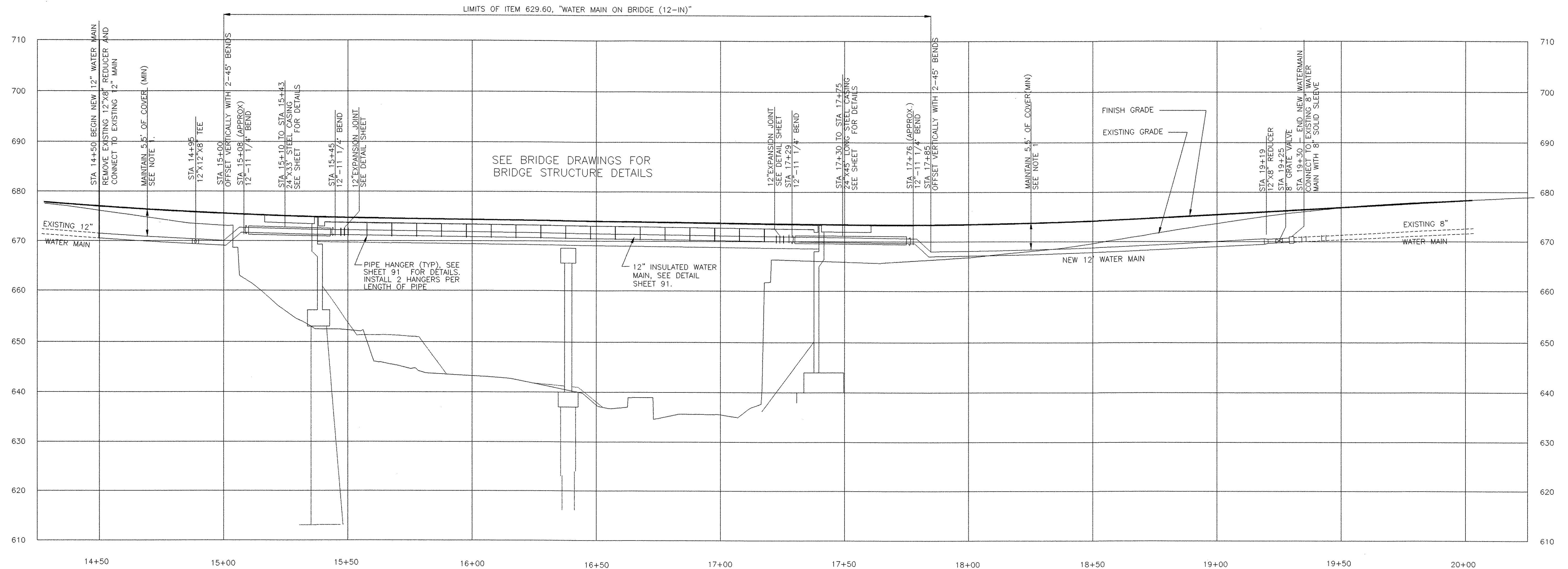
PERMANENT WATER MAIN PROFILE
