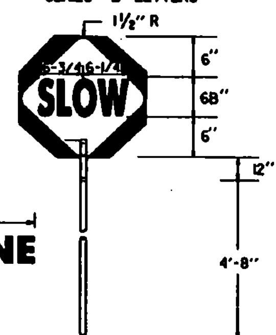
SIGN DETAIL
