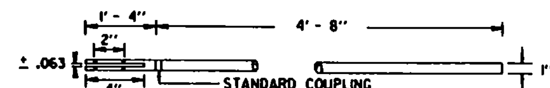
STAFF DETAIL
