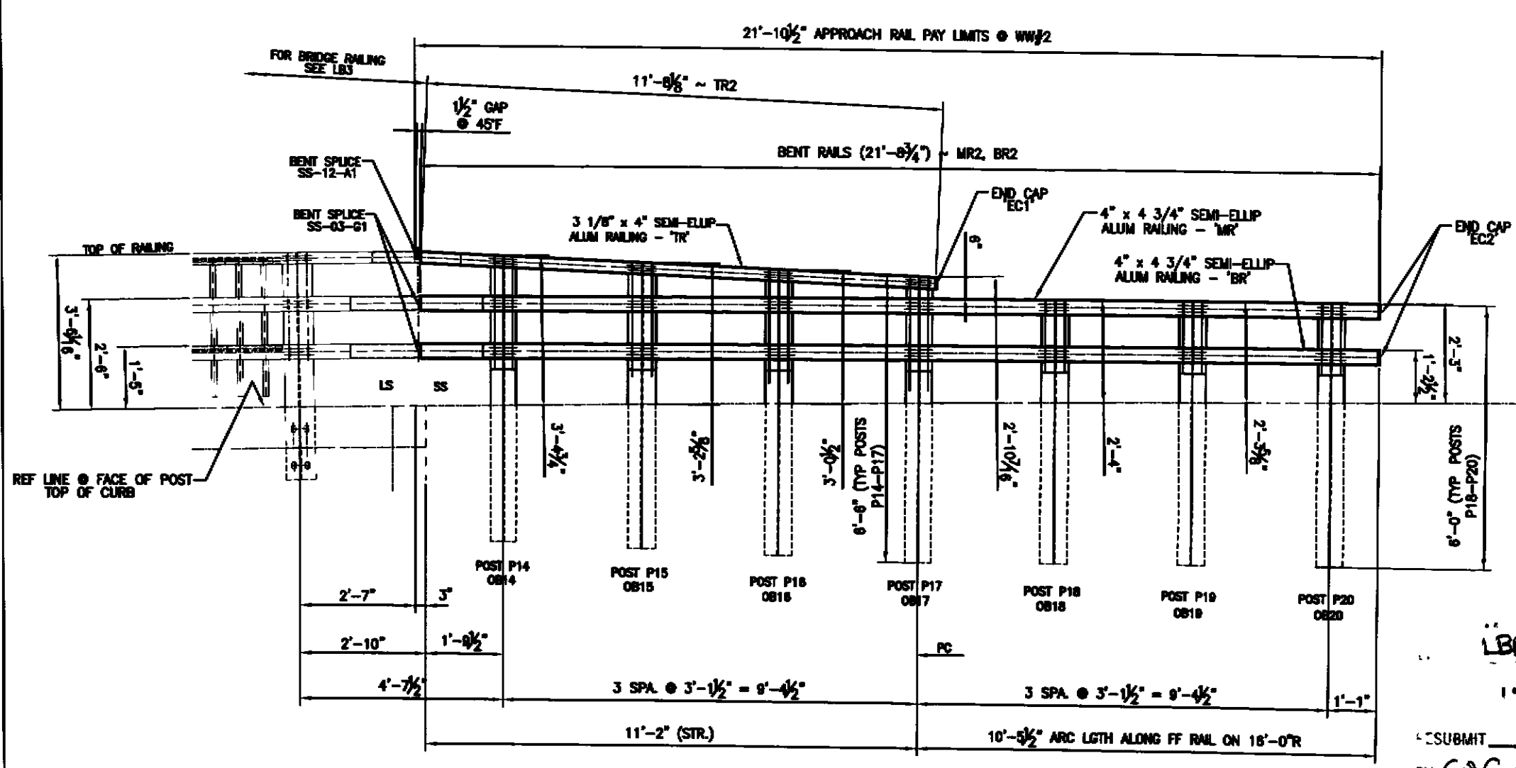
INSIDE ELEVATION OF WW #2 APPROACH RAIL
