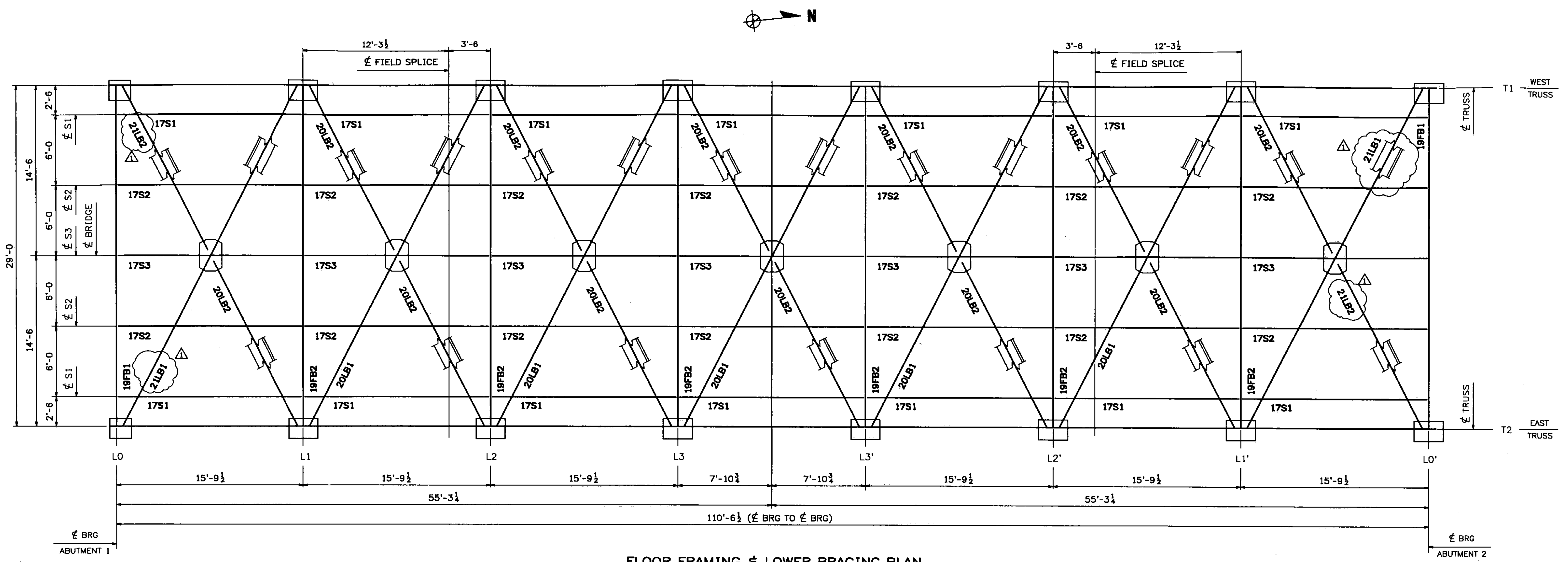
FLOOR FRAMING & LOWER BRACING PLAN
