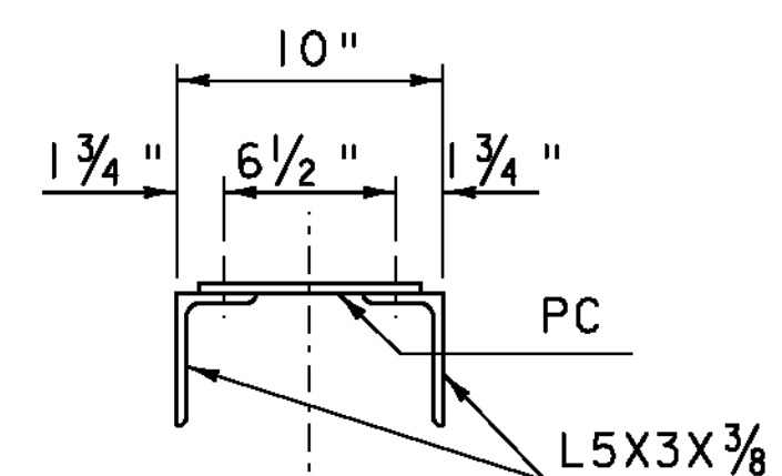
"L3-U2" SECTION
