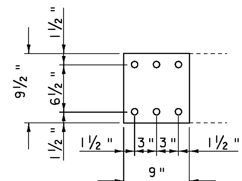
PC DETAIL PL 5/16 x 9 x 9 1/2"
