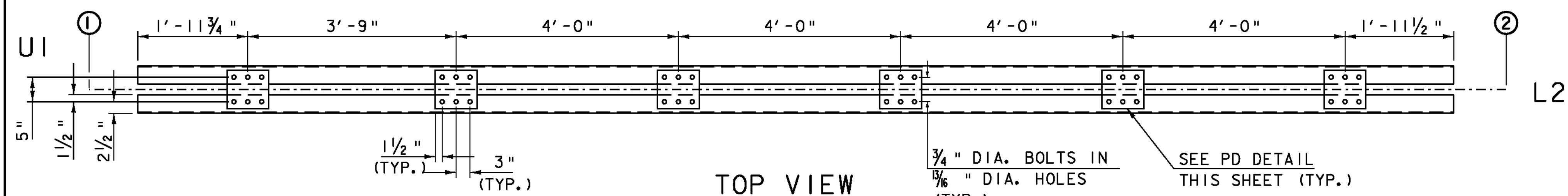
DIAGONAL "L2-U1" 2 - WT4x14x23'-8 1/4" (CVN)
