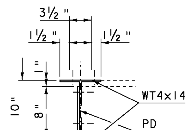
"L2-U1" SECTION
