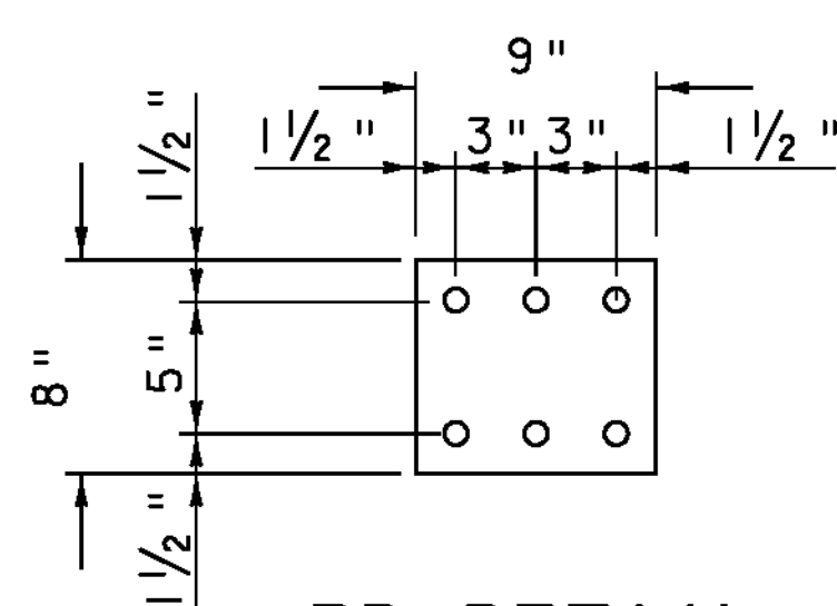
PD DETAIL PL 5/16 x 8 x 9"
